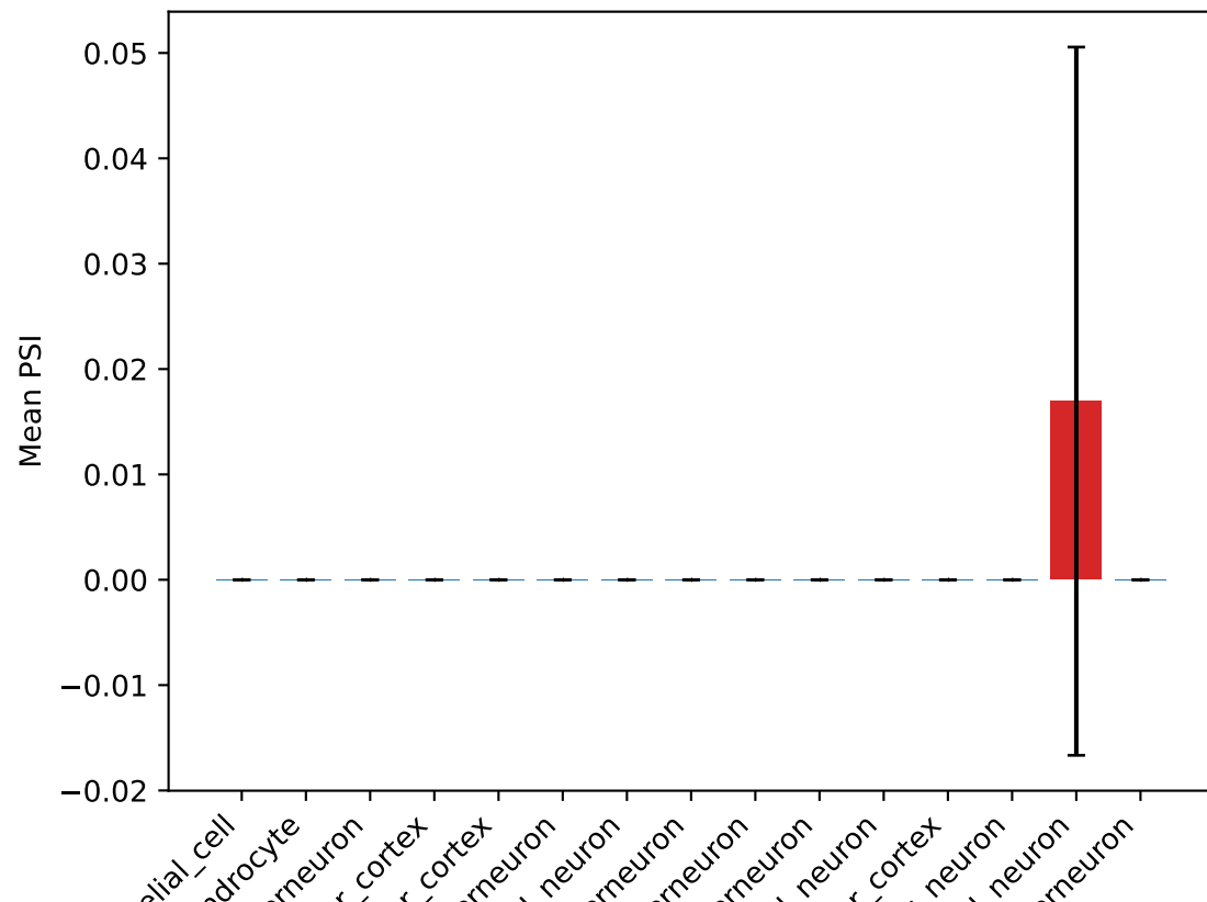
PSI for Garin2 NMD1 exon
