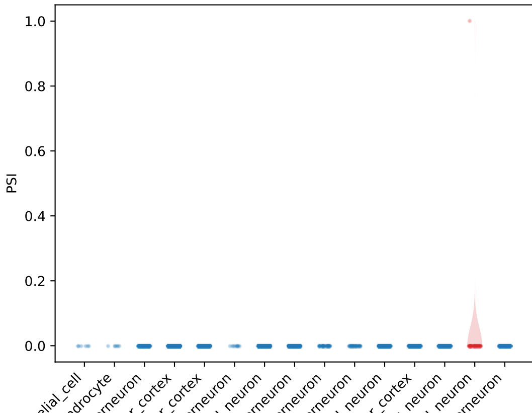
PSI distribution for Garin2 NMD1 exon
