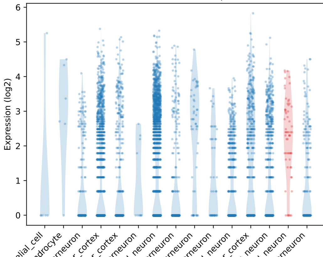
Count distribution for Gpr155
