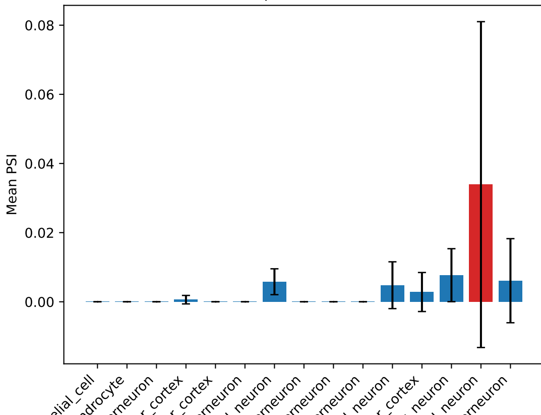
PSI for Gpr155 other1 exon
