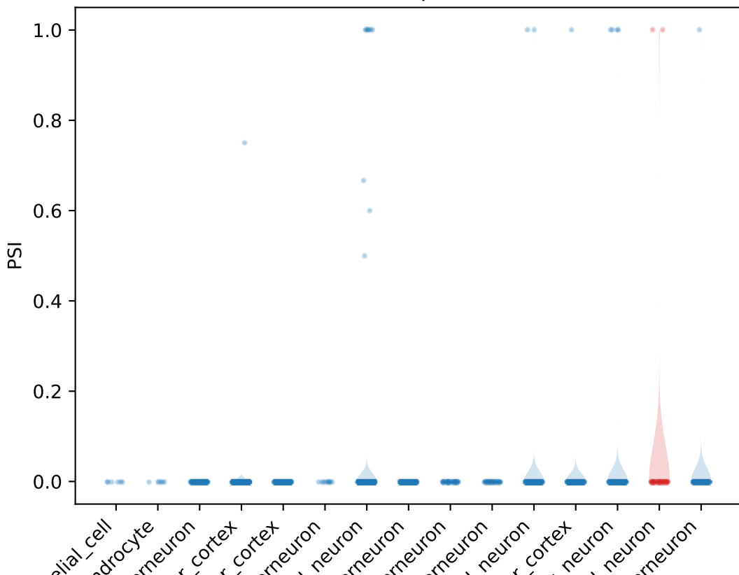
PSI distribution for Gpr155 other1 exon
