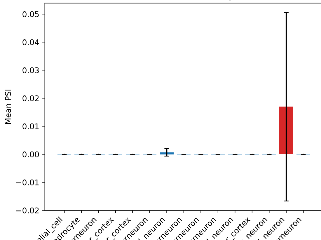
PSI for Lrrc8c ProteinCoding1 exon
