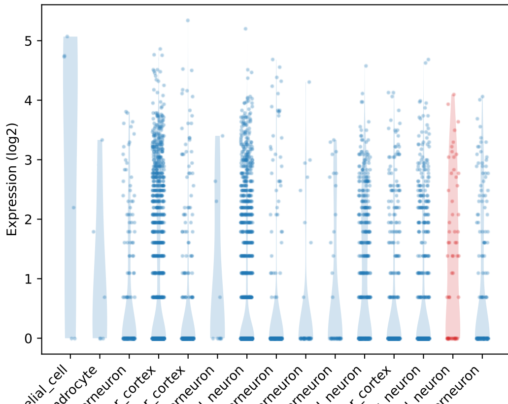
Count distribution for Lrrc8c
