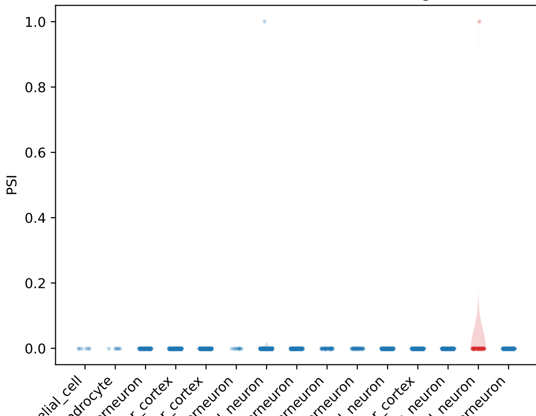
PSI distribution for Lrrc8c ProteinCoding1 exon
