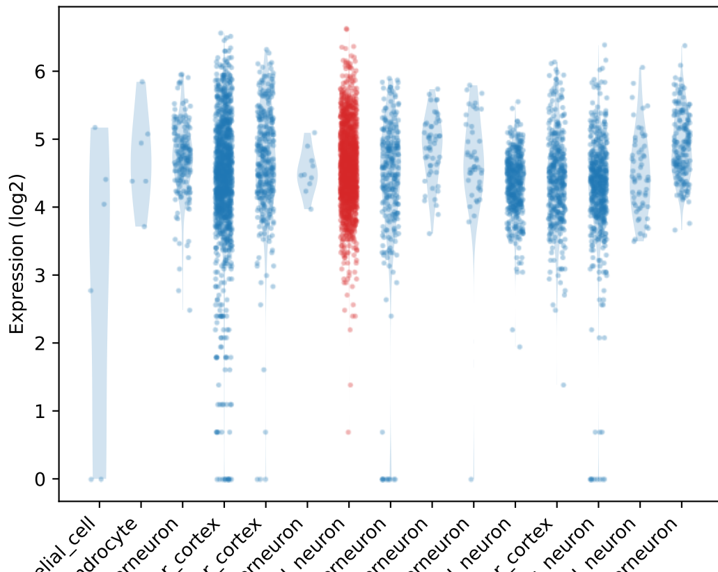
Count distribution for Cnih1
