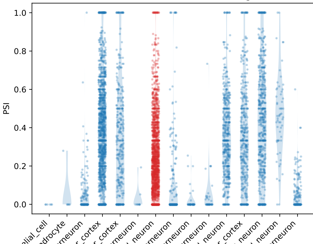
PSI distribution for Cnih1 ProteinCoding1 exon
