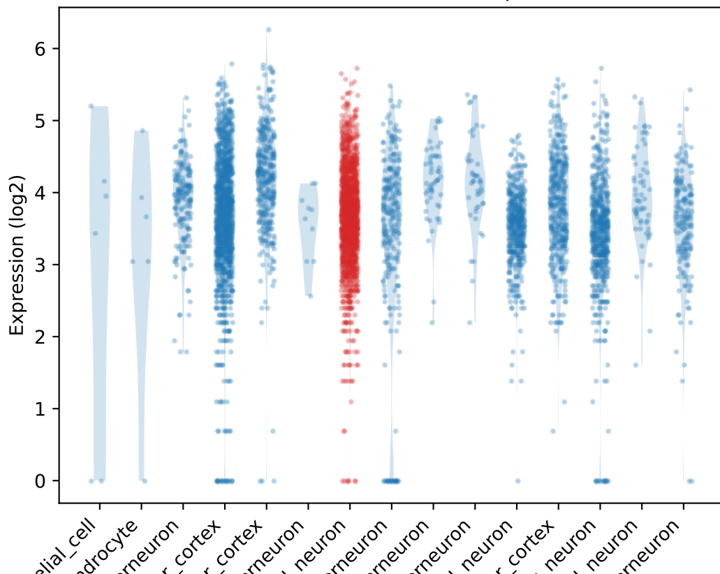
Count distribution for Mrpl13
