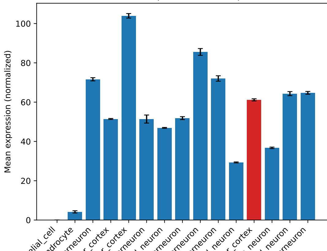
Gene expression for Cadps
