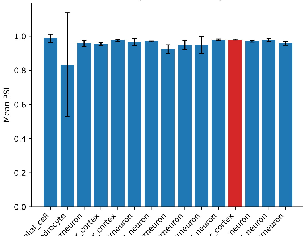
PSI for Sh3bgrl3 ProteinCoding1 exon
