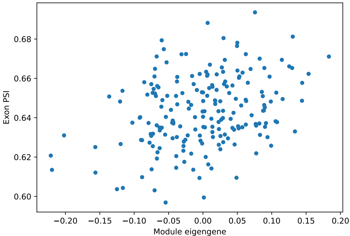
L6b_glutamatergic_cortical_neuron ME vs. PSI for Cldnd1 ProteinCoding2 e Corr: 0.32
