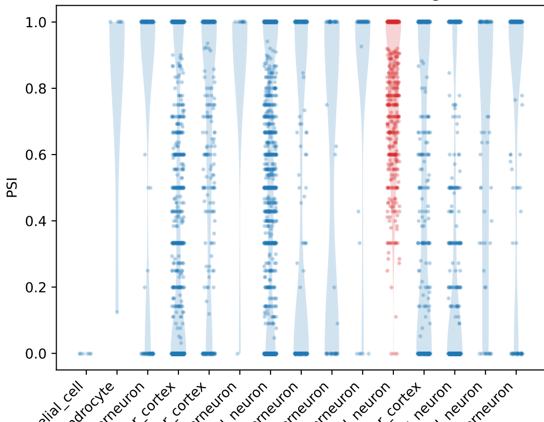
PSI distribution for Cldnd1 ProteinCoding2 exon
