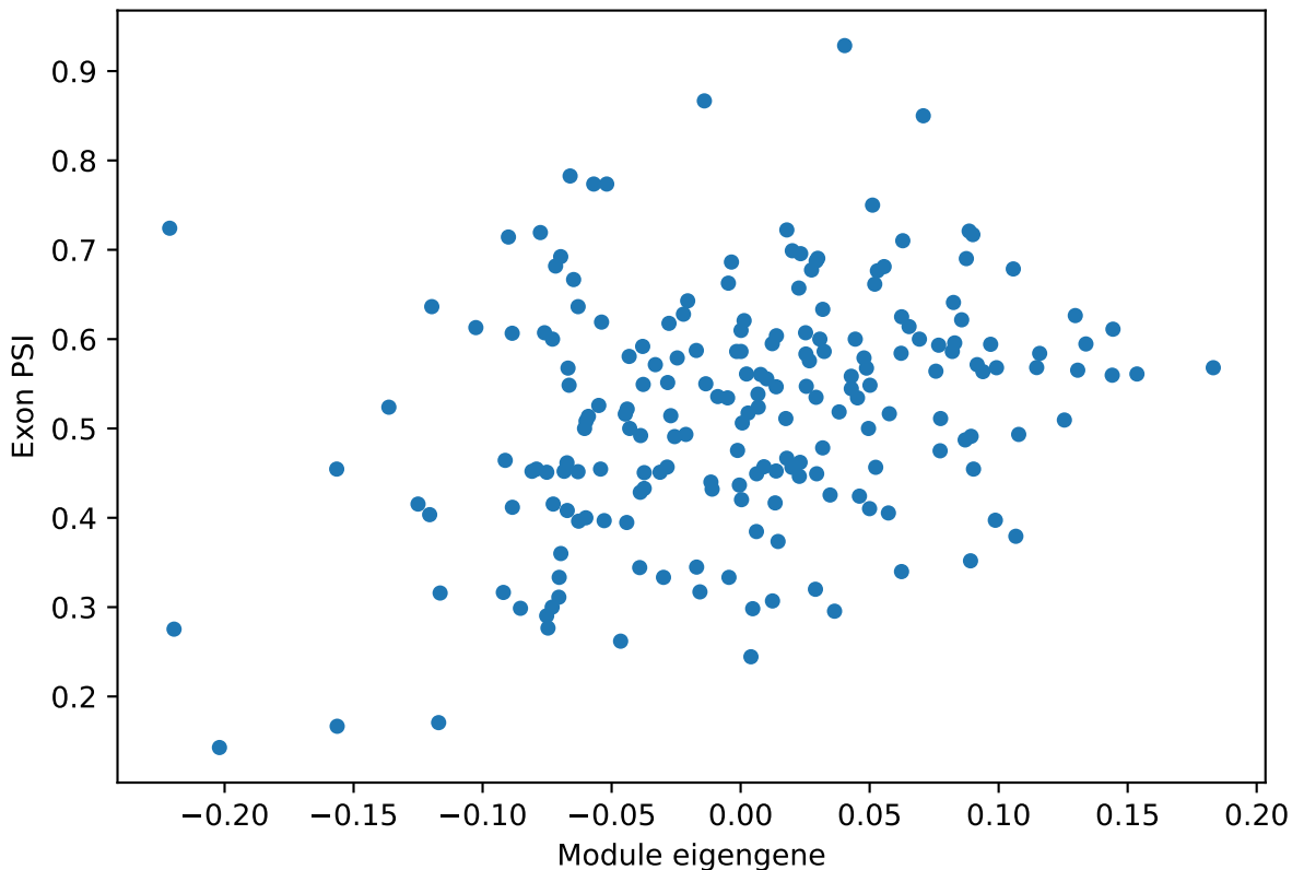
L6b_glutamatergic_cortical_neuron ME vs. PSI for Fzd10os other6 exon Corr: 0.3
