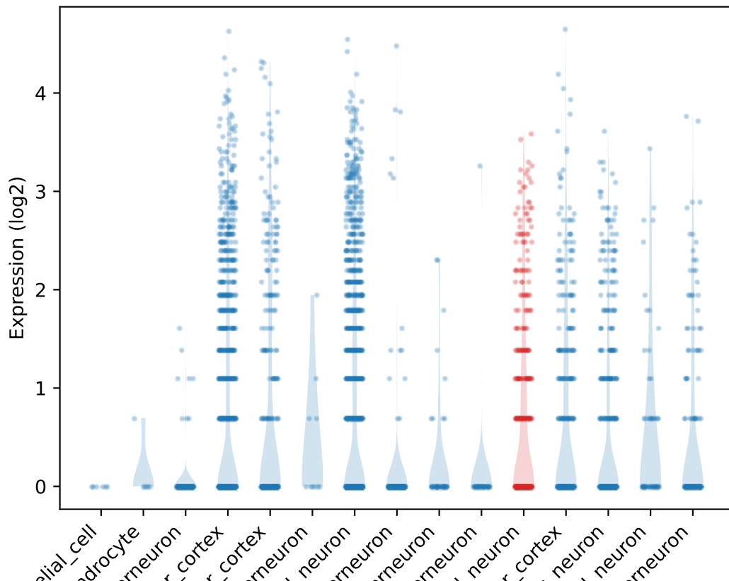
Count distribution for Ptchd1
