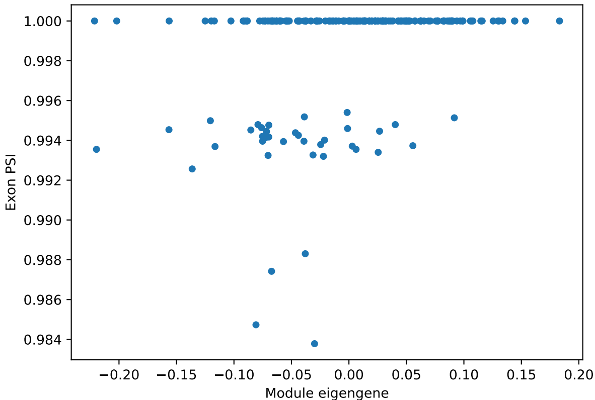
L6b_glutamatergic_cortical_neuron ME vs. PSI for Ptchd1 ProteinCoding1 e Corr: 0.31
