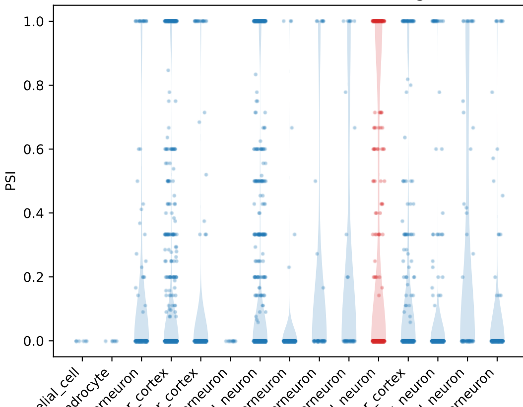
PSI distribution for Rmnd1 ProteinCoding2 exon
