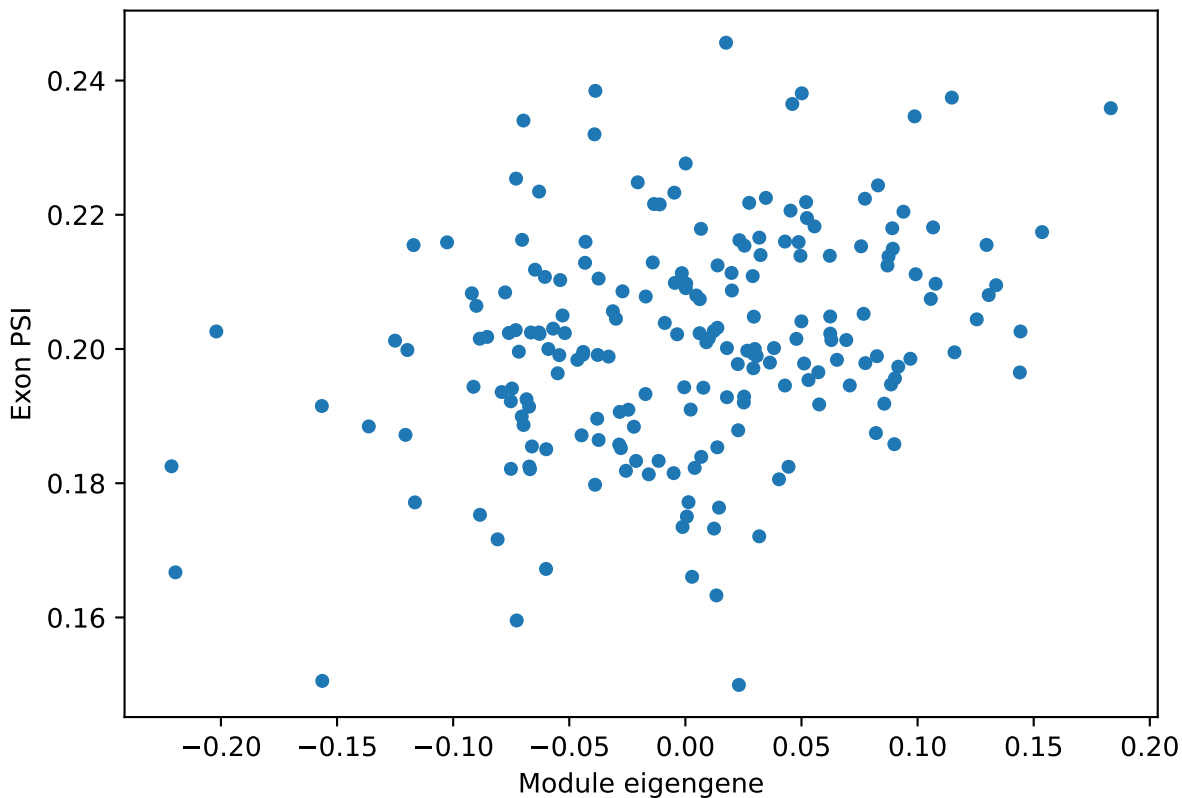
L6b_glutamatergic_cortical_neuron ME vs. PSI for Rmnd1 ProteinCoding2 e Corr: 0.31
