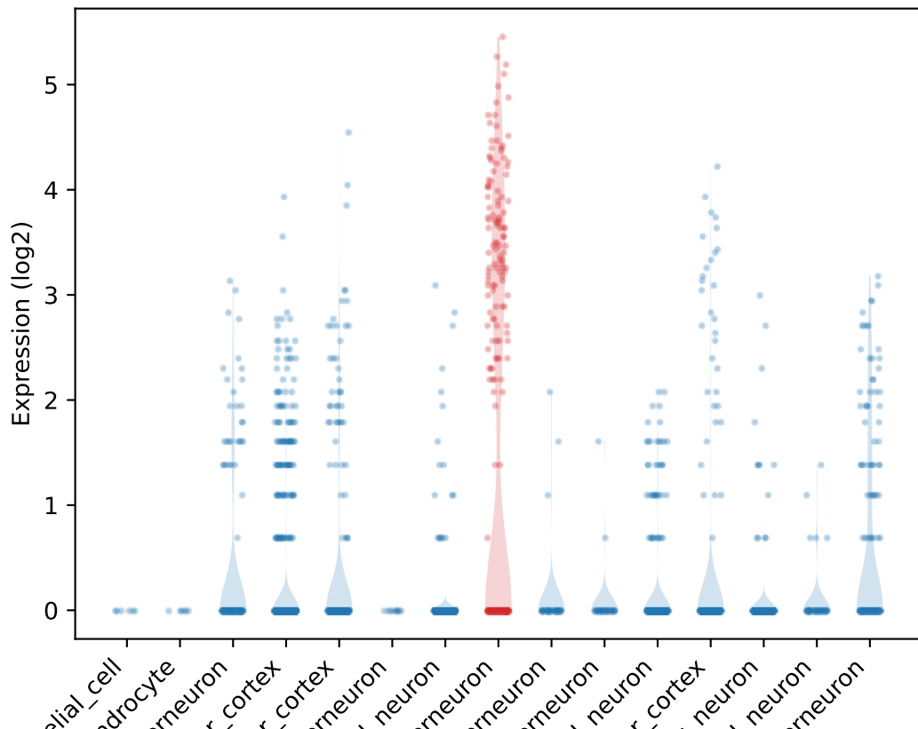
Count distribution for Crlf1
