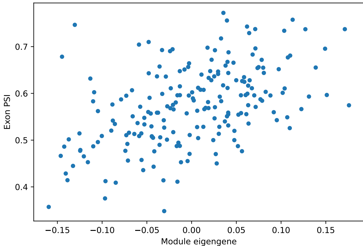
VIP_GABAergic_cortical_interneuron ME vs. PSI for Cr1f1 ProteinCoding2 ex Corr: 0.49
