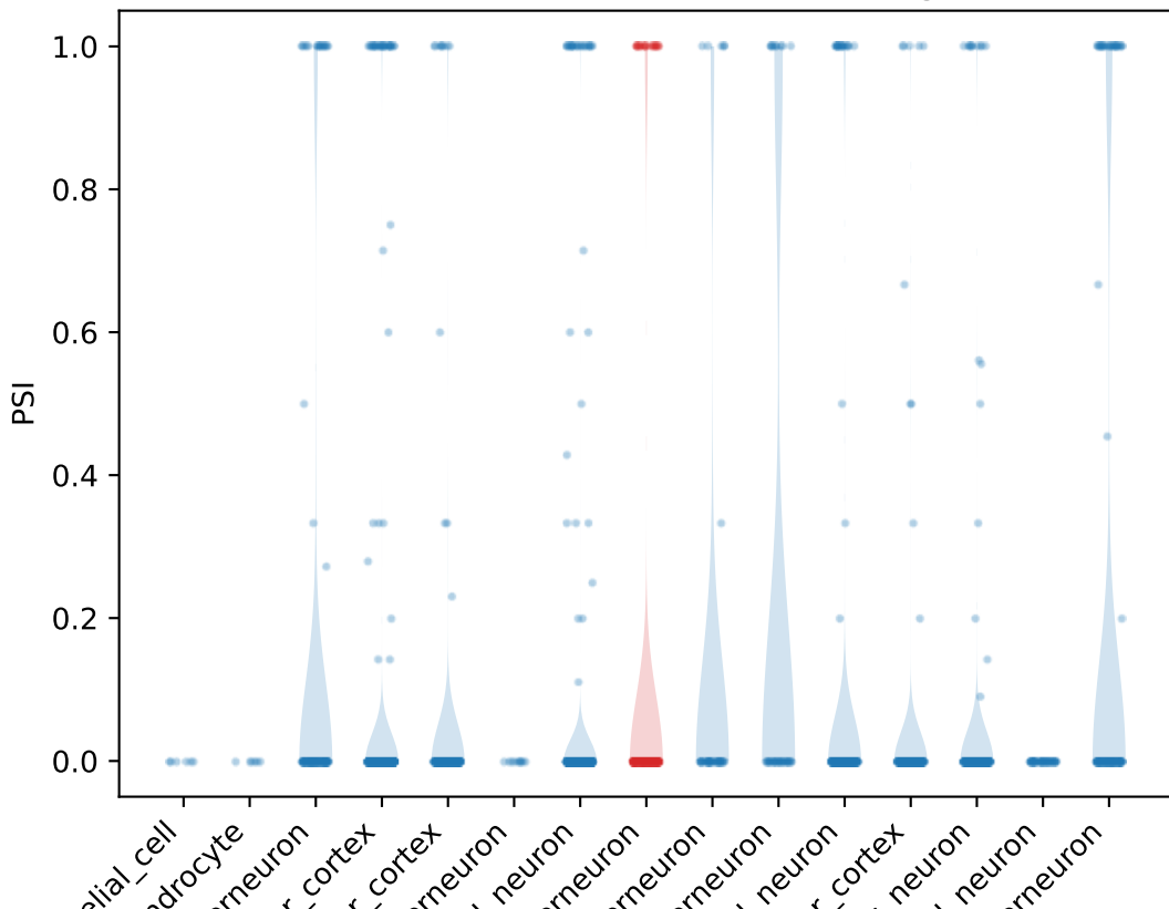
PSI distribution for Exoc1 ProteinCoding2 exon
