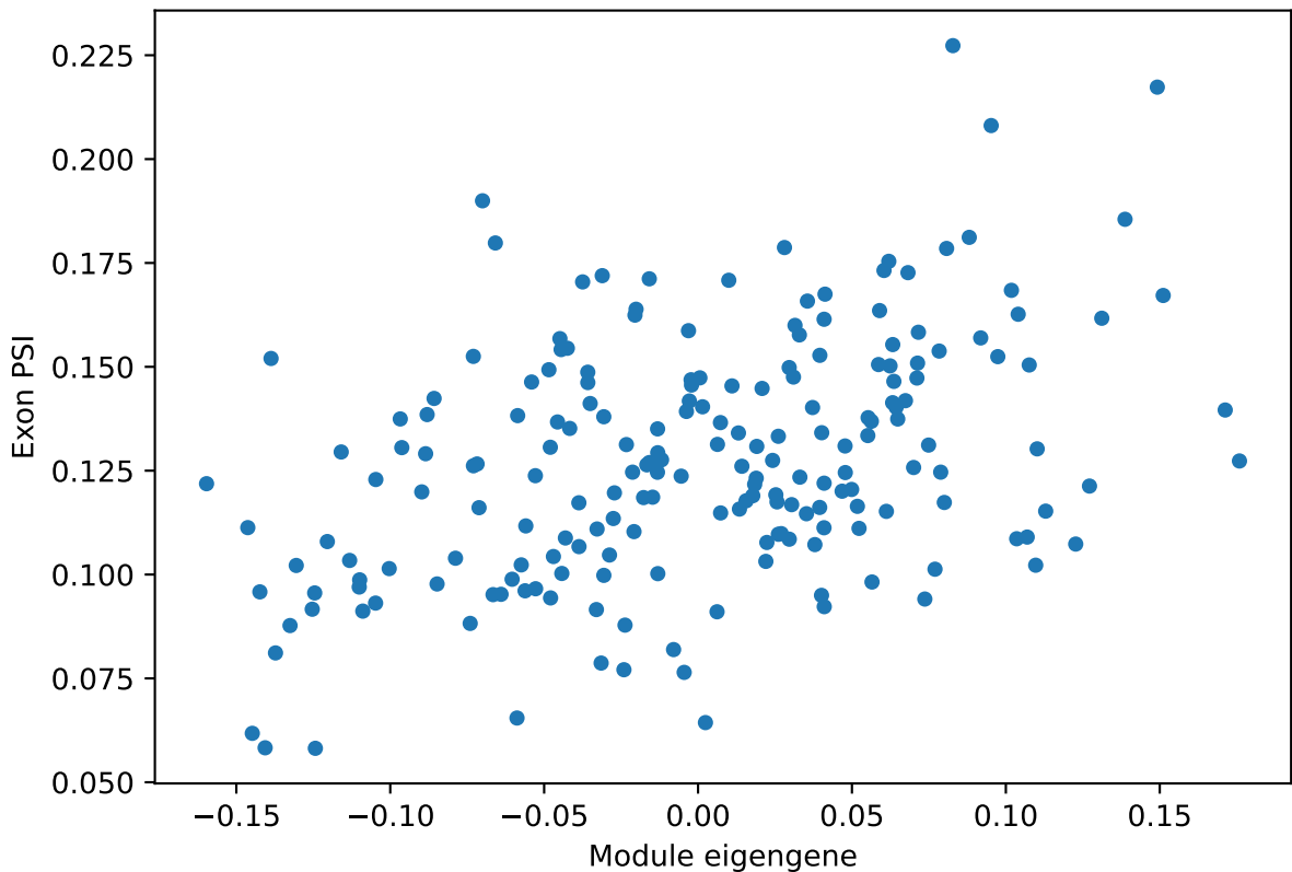
VIP_GABAergic_cortical_interneuron ME vs. PSI for Exoc1 ProteinCoding2 Corr: 0.42
