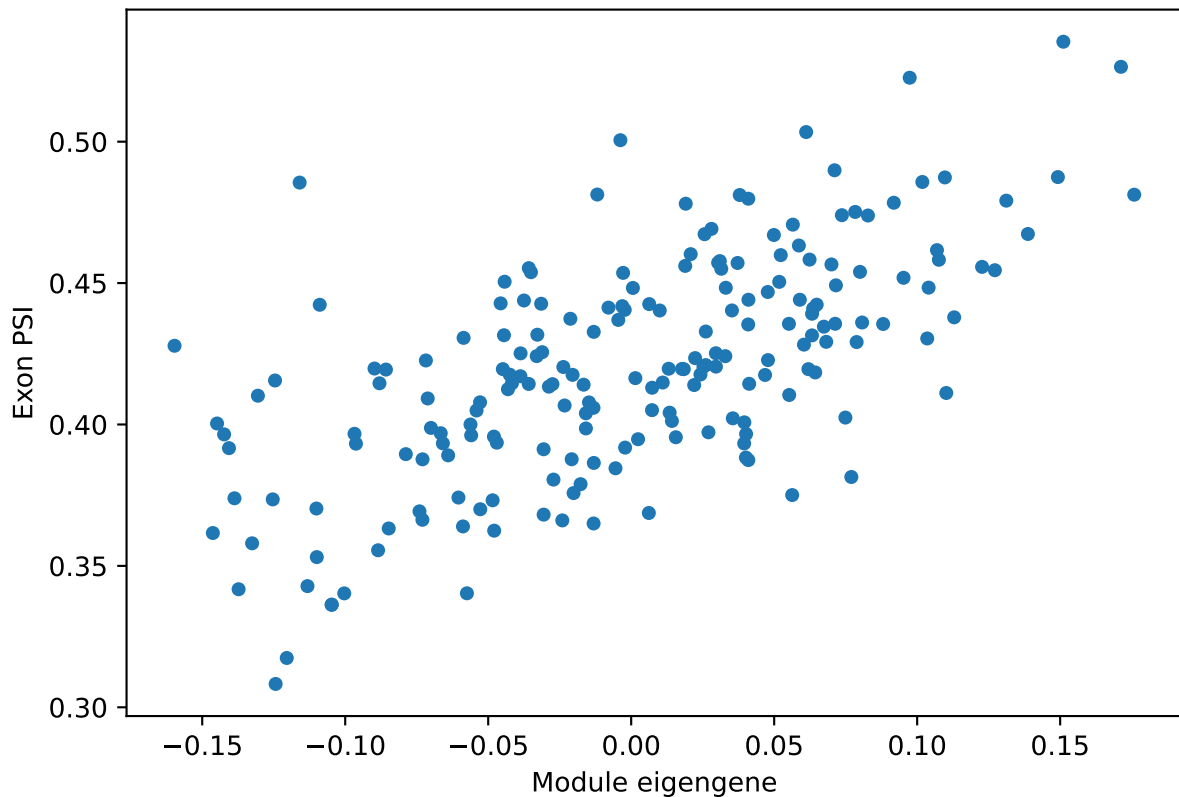
VIP_GABAergic_cortical_interneuron ME vs. PSI for Fhl1 ProteinCoding2 ex Corr: 0.65
