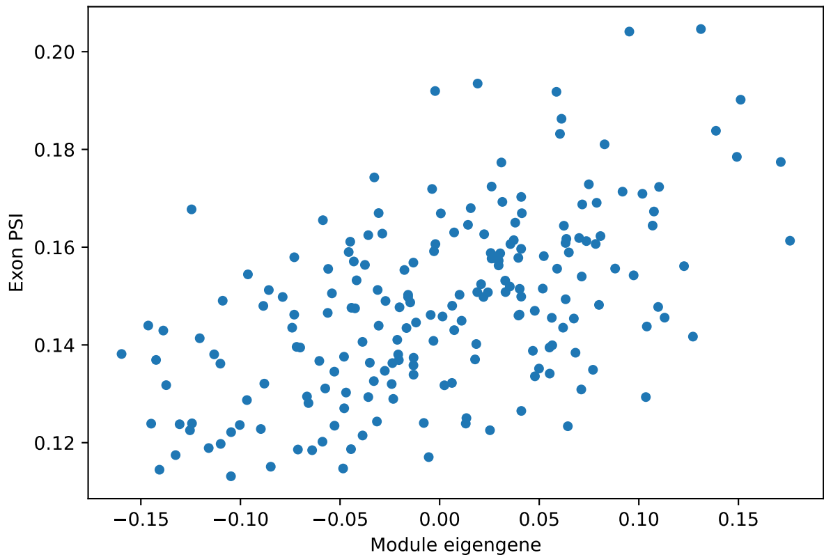
VIP_GABAergic_cortical_interneuron ME vs. PSI for Nr1x1 ProteinCoding1 e Corr: 0.54
