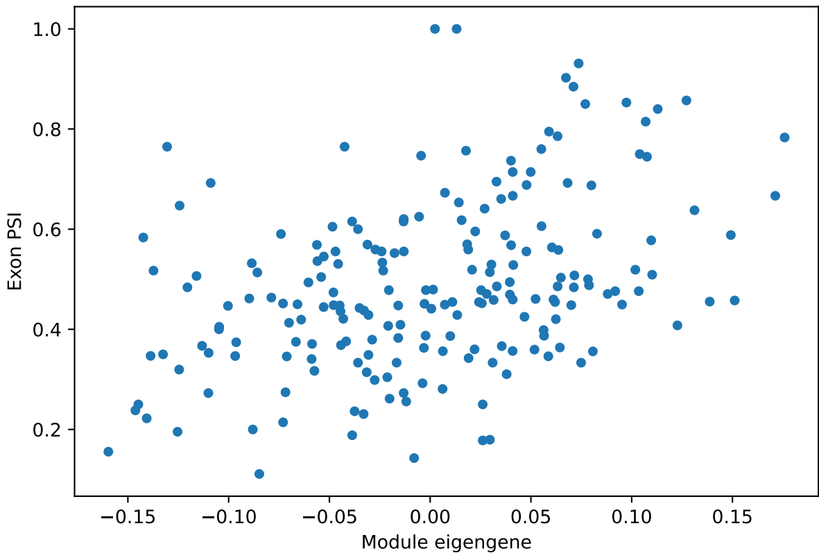
VIP_GABAergic_cortical_interneuron ME vs. PSI for Sox2ot other1 exon Corr: 0.4
