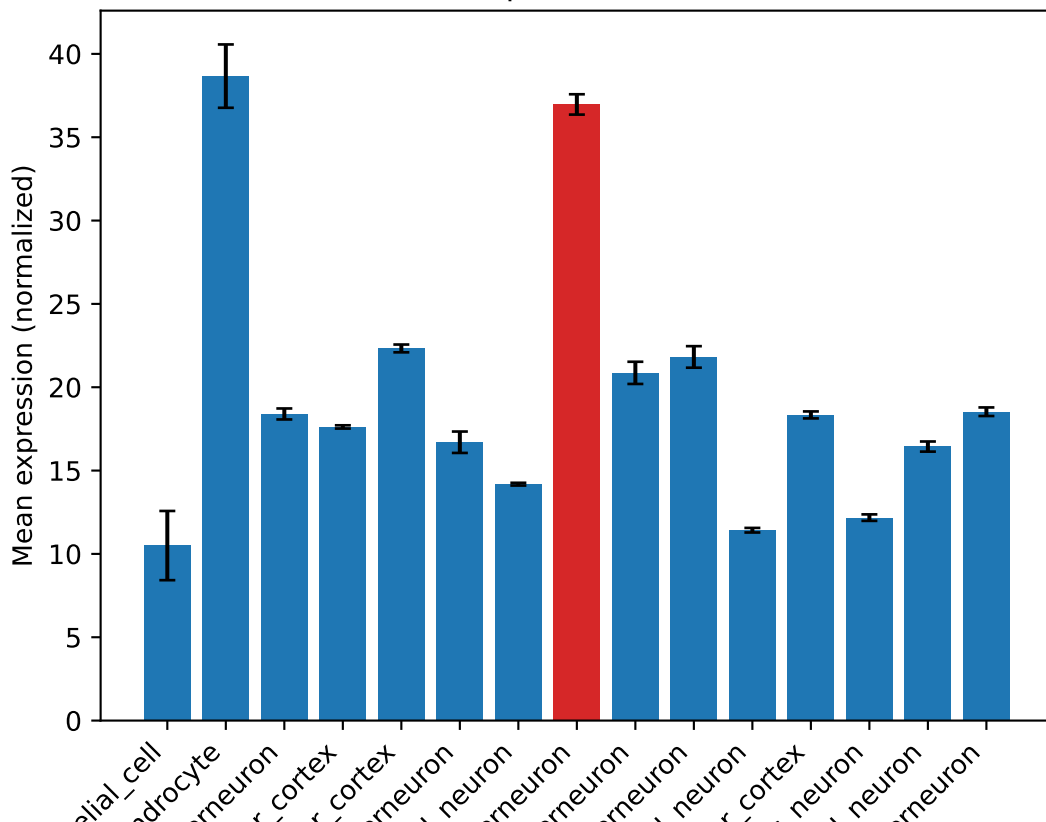
Gene expression for Tial1
