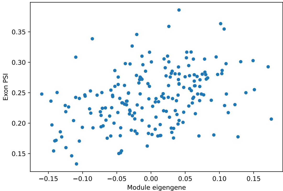
VIP_GABAergic_cortical_interneuron ME vs. PSI for Tial1 NMD1 exon Corr: 0.38
