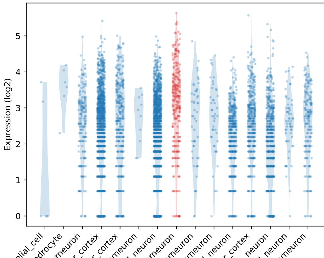
Count distribution for Tial1
