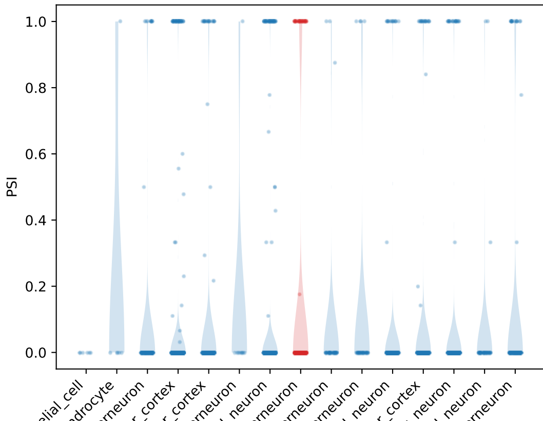
PSI distribution for Tial1 NMD1 exon
