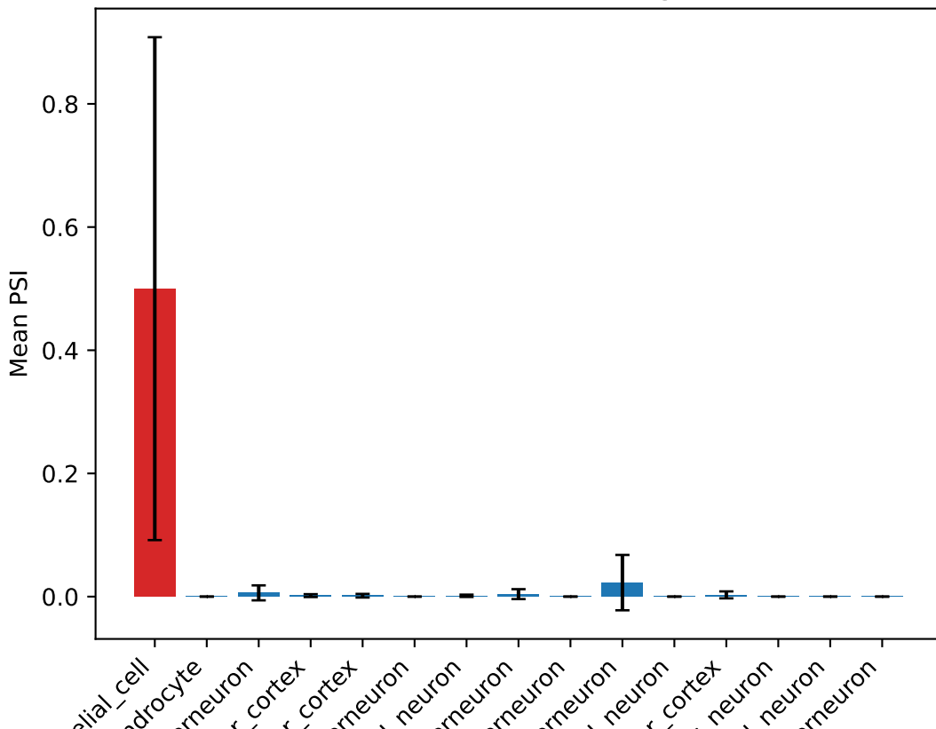
PSI for Ablim1 ProteinCoding1 exon
