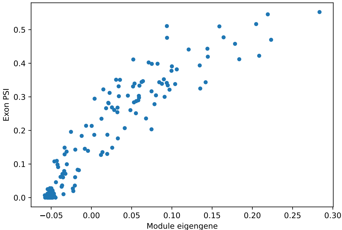
endothelial_cell ME vs. PSI for Ablim1 ProteinCoding1 exon Corr: 0.94
