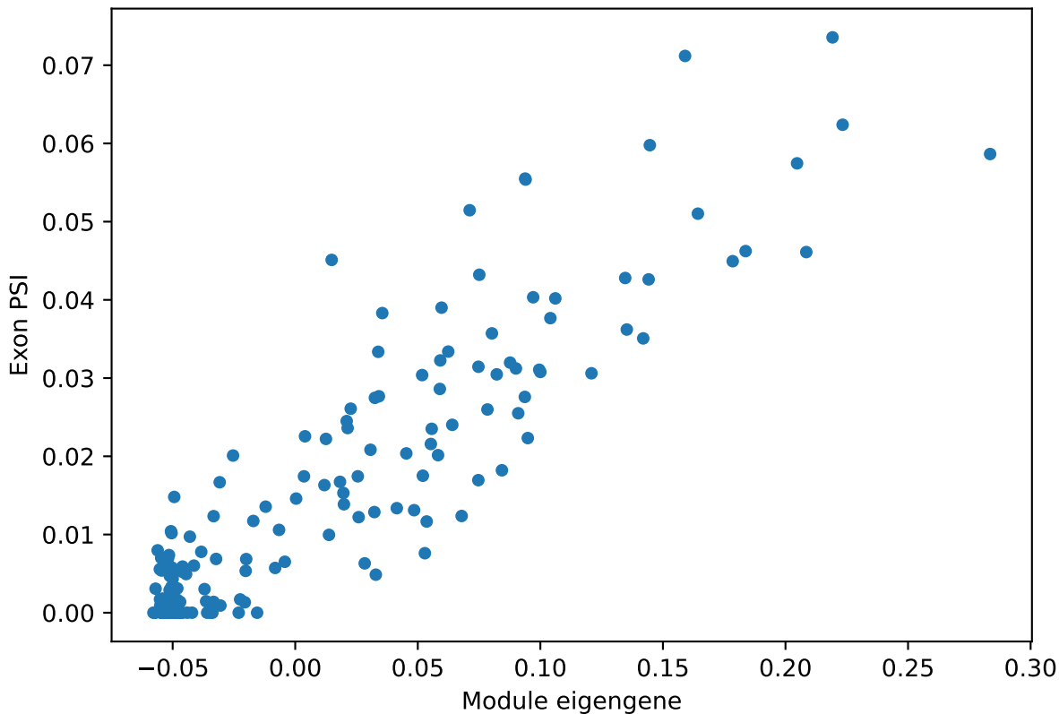
endothelial_cell ME vs. PSI for Cep164 ProteinCoding5 exon Corr: 0.91
