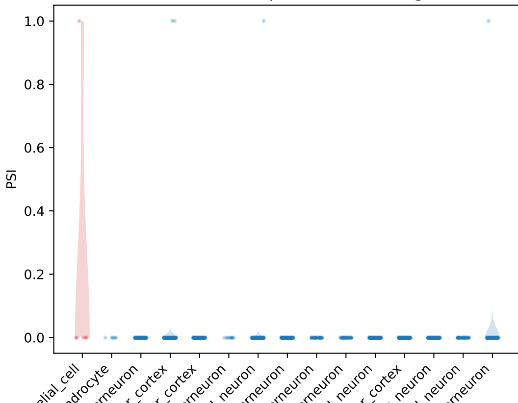
PSI distribution for Cep164 ProteinCoding5 exon
