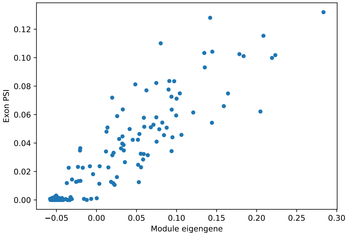
endothelial_cell ME vs. PSI for Clip1 ProteinCoding6 exon Corr: 0.92
