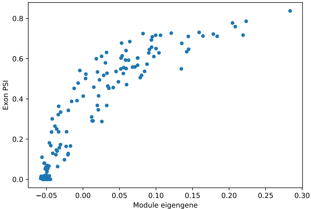
endothelial_cell ME vs. PSI for Mpzl1 ProteinCoding1 exon Corr: 0.91
