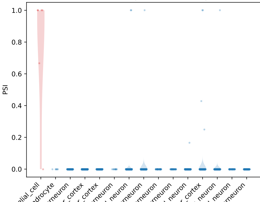
PSI distribution for Mpzl1 ProteinCoding1 exon
