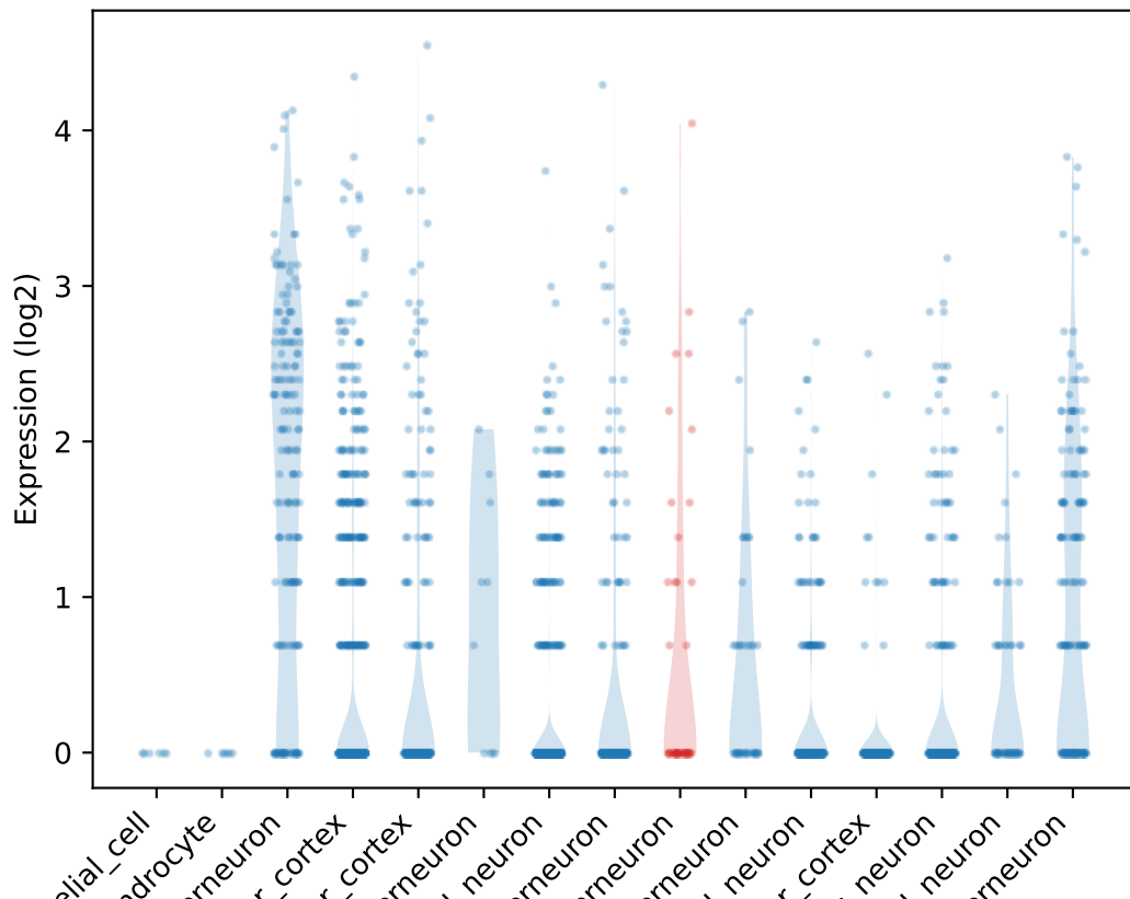
Count distribution for Ank1
