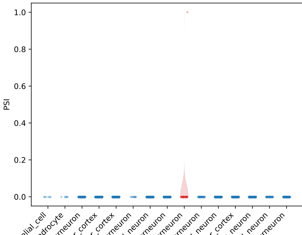
PSI distribution for Ank1 NMD1 exon
