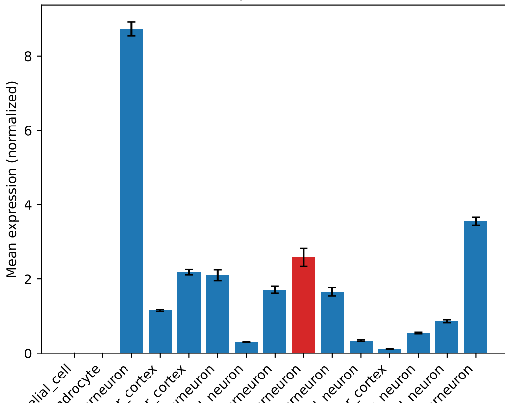
Gene expression for Ank1
