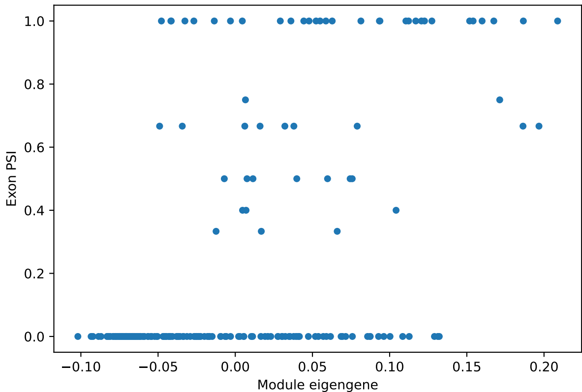
lamp5_GABAergic_cortical_interneuron ME vs. PSI for Ank1 NMD1 exon Corr: 0.53
