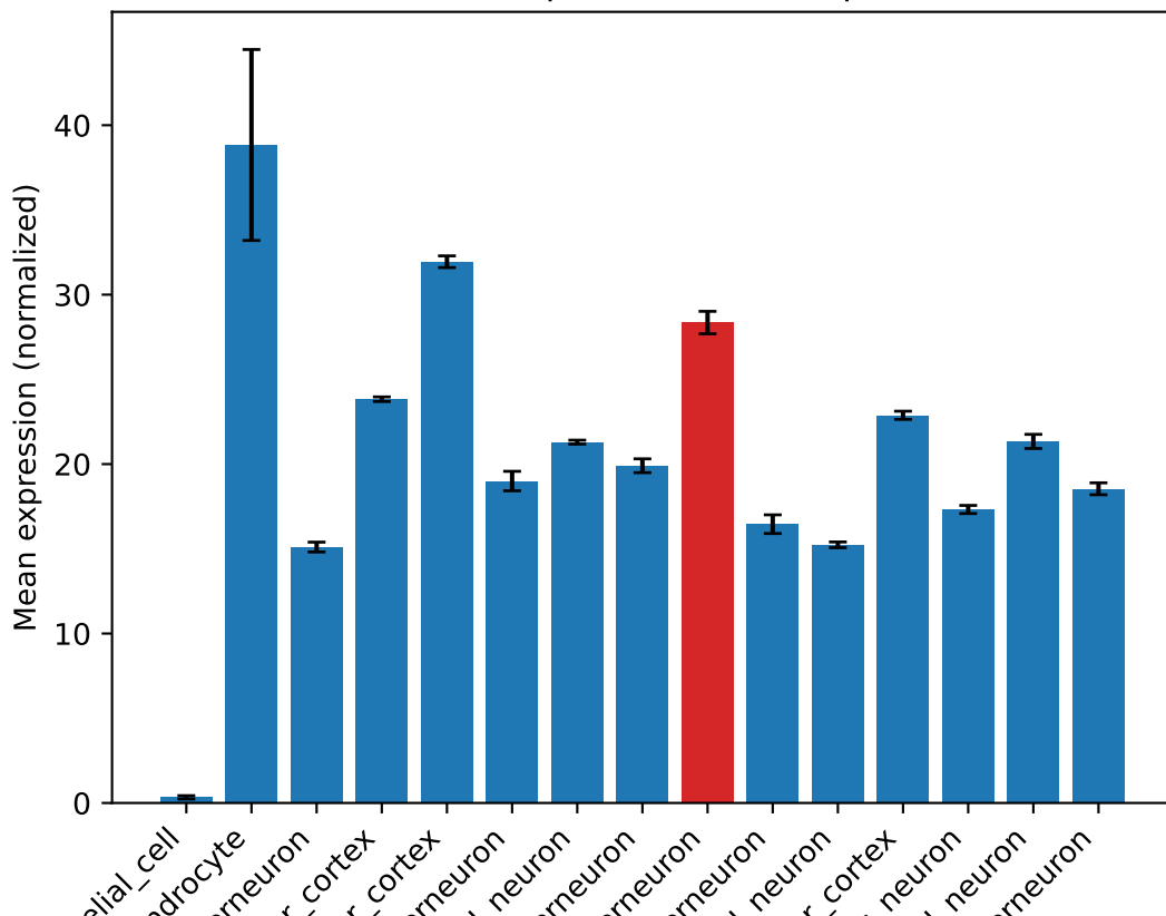
Gene expression for Clasp2
