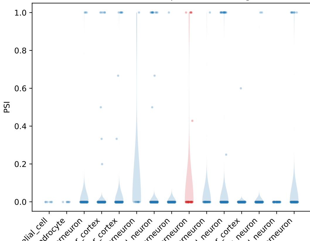
PSI distribution for Clasp2 ProteinCoding1 exon
