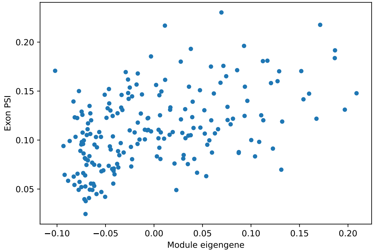
lamp5_GABAergic_cortical_interneuron ME vs. PSI for Clasp2 ProteinCoding3 Corr: 0.48
