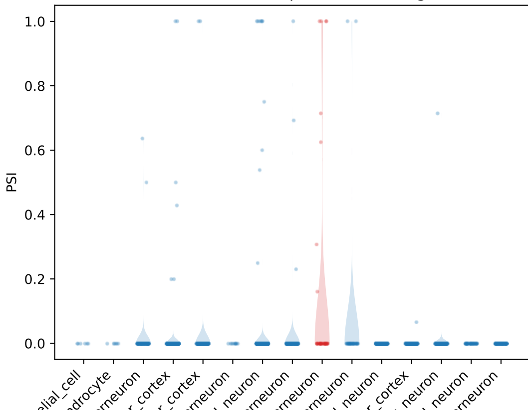
PSI distribution for Lrrfip1 ProteinCoding3 exon
