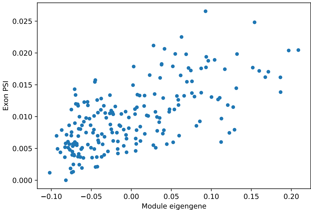
lamp5_GABAergic_cortical_interneuron ME vs. PSI for Lrrfip1 ProteinCoding Corr: 0.66
