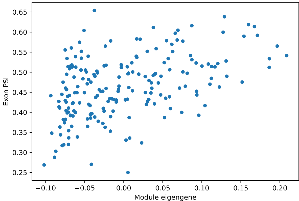
lamp5_GABAergic_cortical_interneuron ME vs. PSI for Nrnx3 ProteinCoding4 Corr: 0.46
