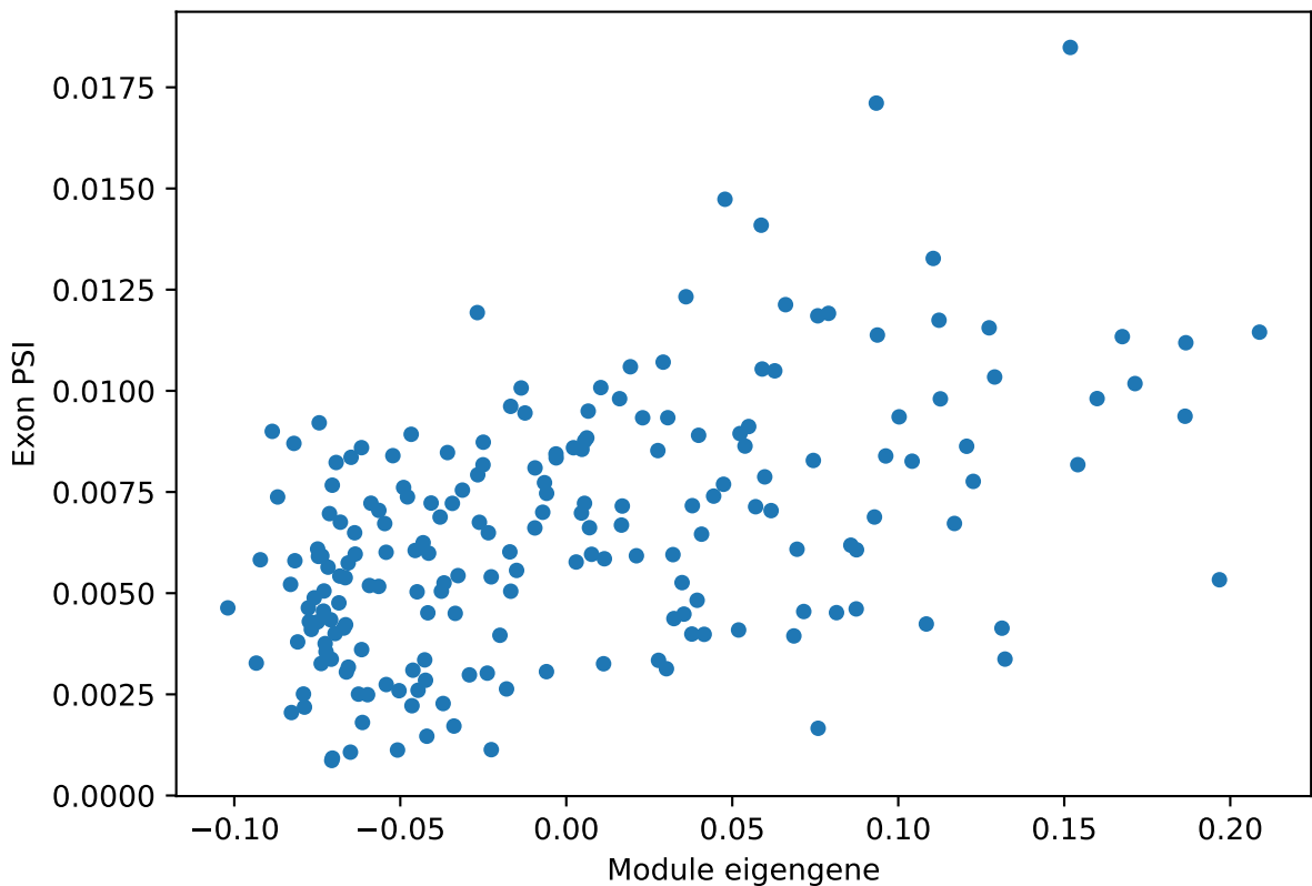
lamp5_GABAergic_cortical_interneuron ME vs. PSI for Pigk ProteinCoding2 Corr: 0.5
