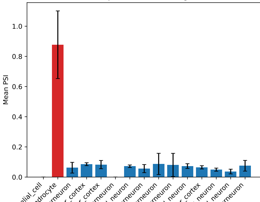
PSI for Gpm6b ProteinCoding2 exon
