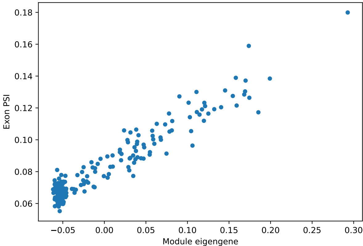
oligodendrocyte ME vs. PSI for Gpm6b ProteinCoding2 exon Corr: 0.96
