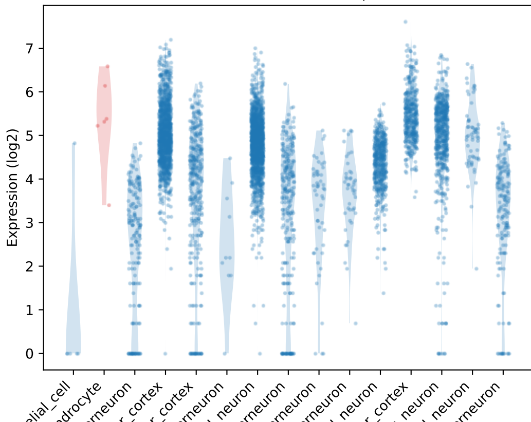
Count distribution for Gpm6b
