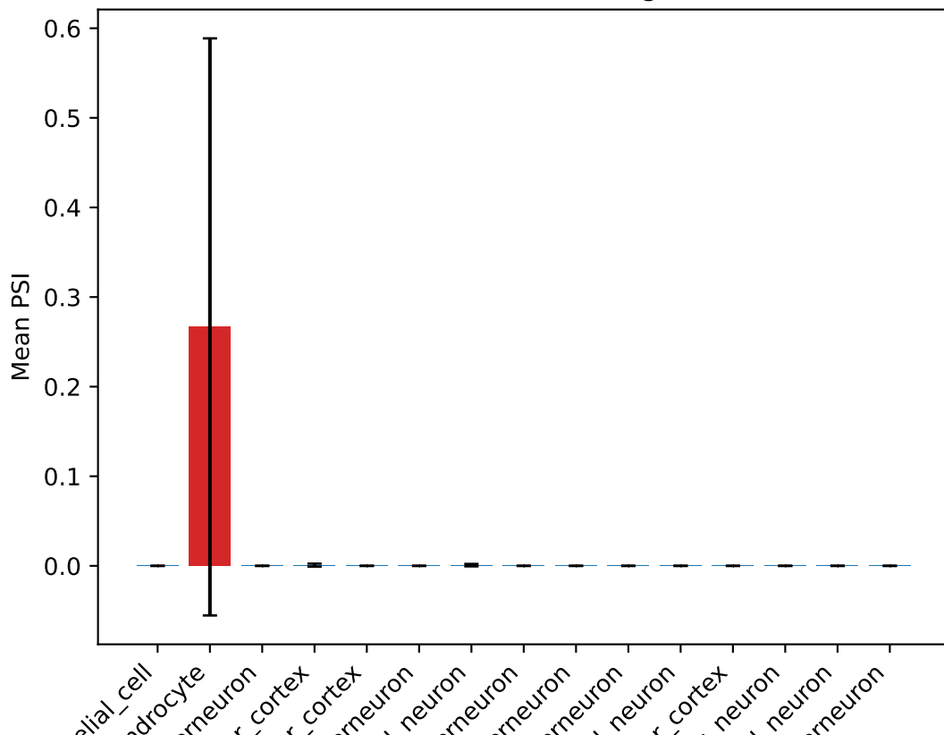
PSI for Gsn ProteinCoding4 exon
