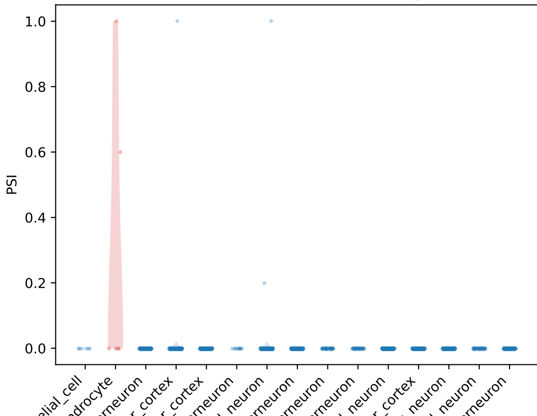
PSI distribution for Gsn ProteinCoding4 exon
