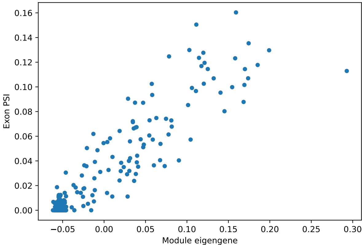
oligodendrocyte ME vs. PSI for Gsn ProteinCoding4 exon Corr: 0.92
