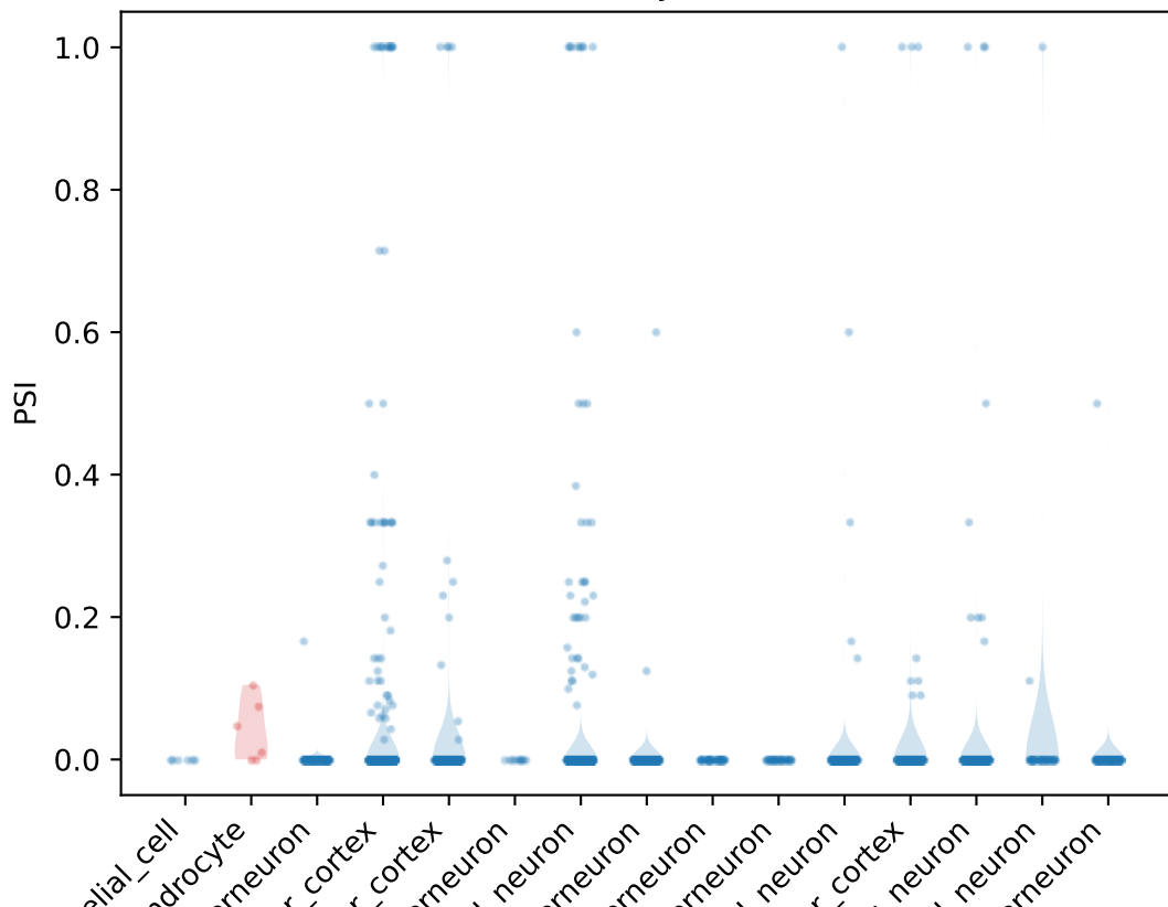
PSI distribution for Jsd2 NMD3 exon
