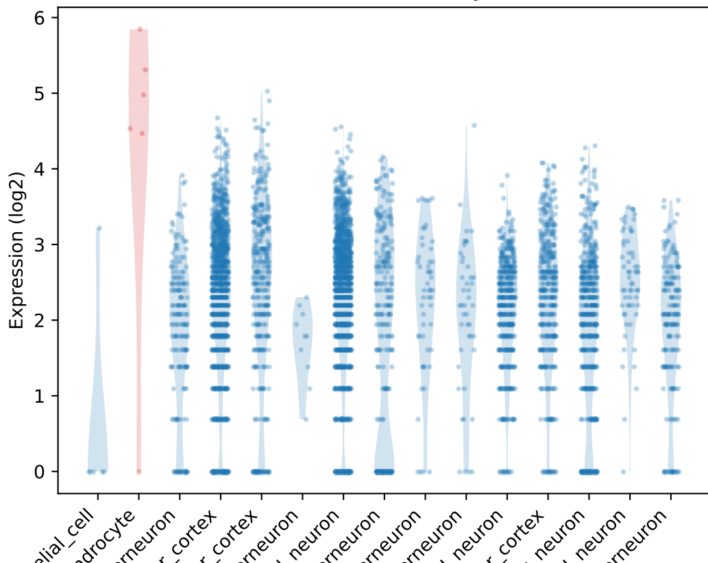
Count distribution for Josd2
