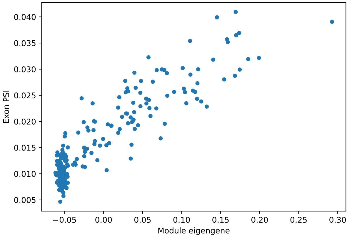
oligodendrocyte ME vs. PSI for Jost2 NMD3 exon Corr: 0.91
