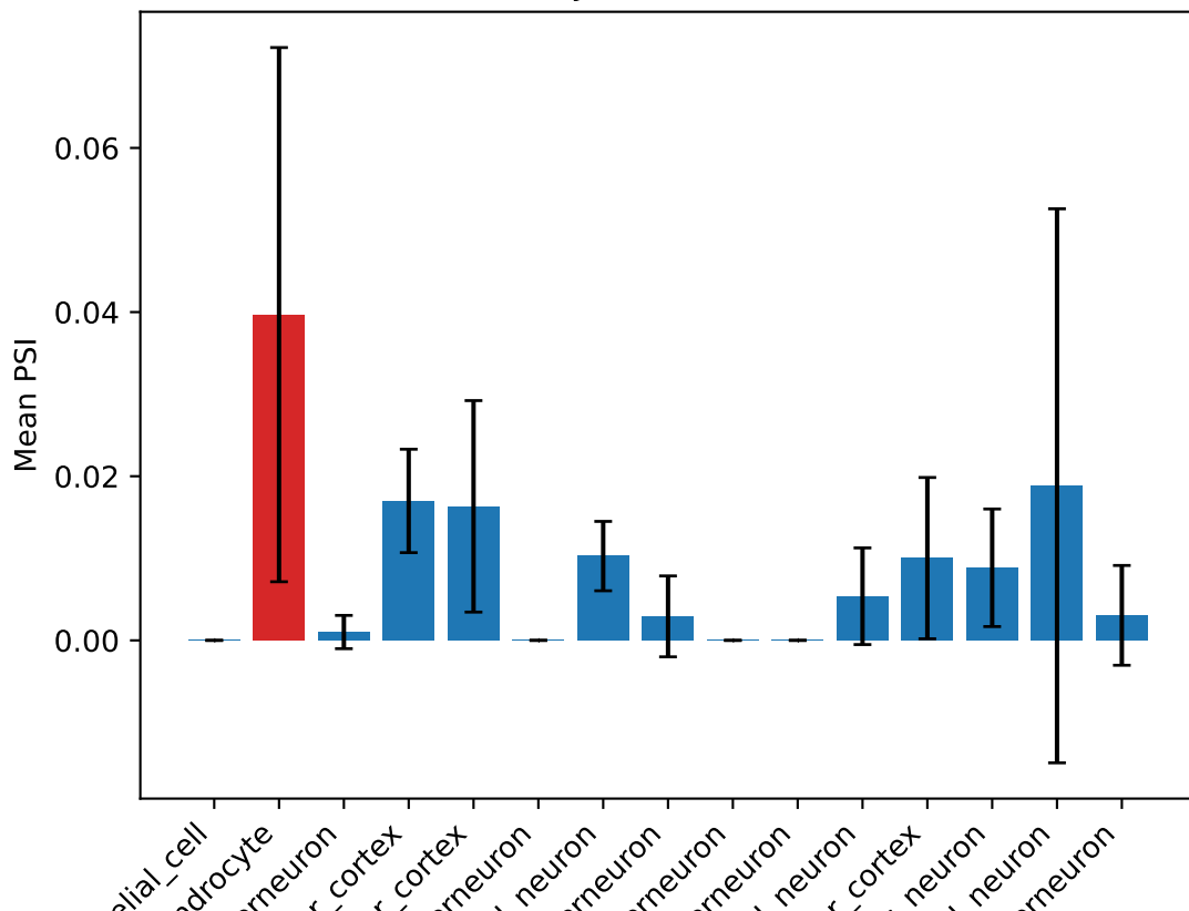
PSI for Jostd2 NMD3 exon
