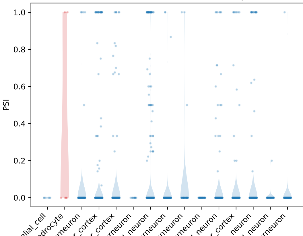
PSI distribution for Nkain4 ProteinCoding1 exon
