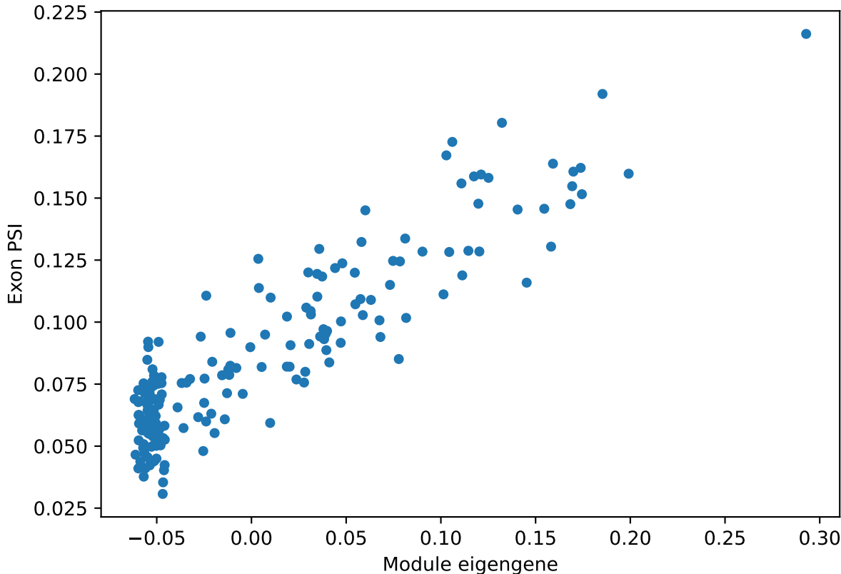
oligodendrocyte ME vs. PSI for Nkain4 ProteinCoding1 exon Corr: 0.91
