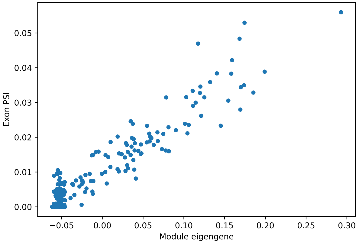
oligodendrocyte ME vs. PSI for Tmem63b ProteinCoding1 exon Corr: 0.95
