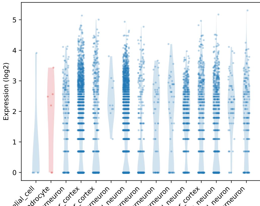
Count distribution for Tmem63b
