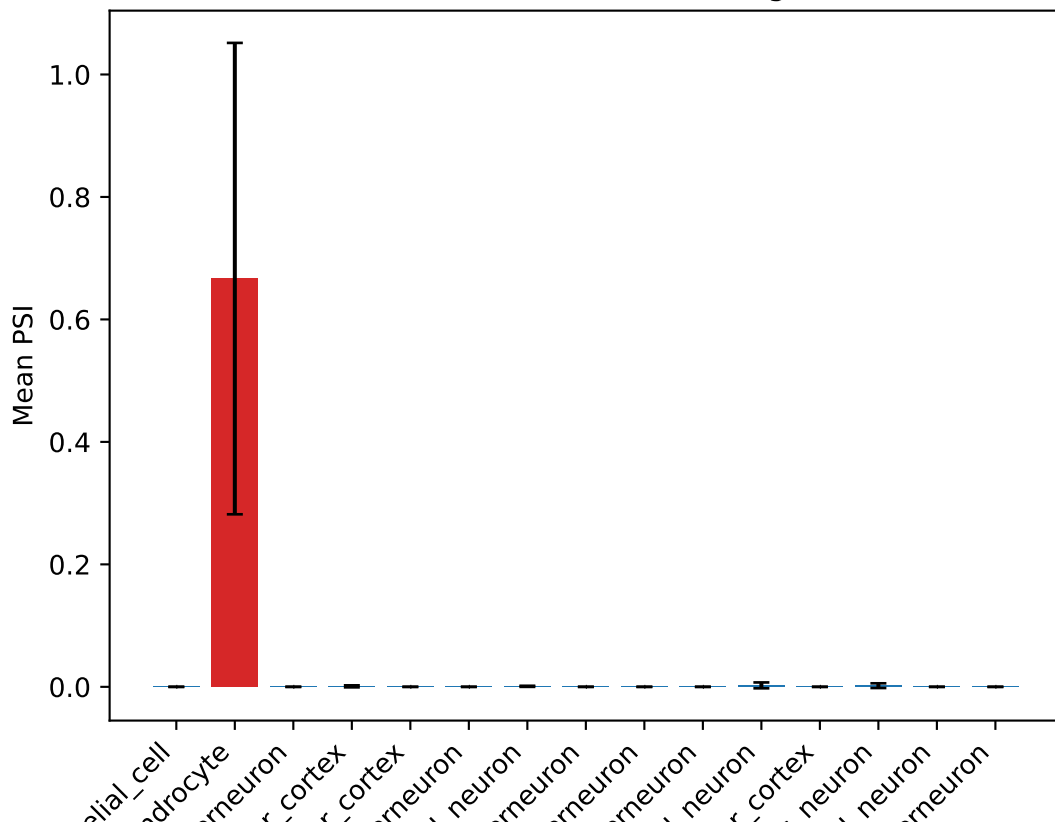
PSI for Tmem63b ProteinCoding1 exon
