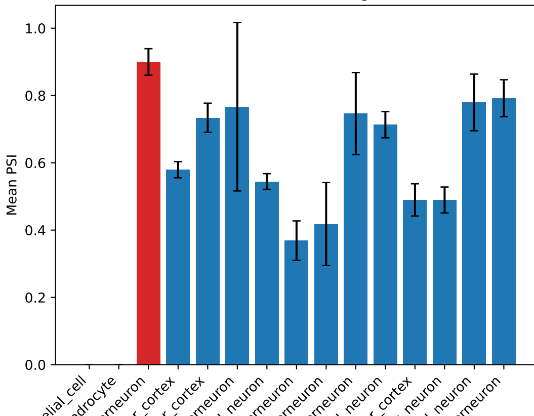
PSI for Mff ProteinCoding7 exon
