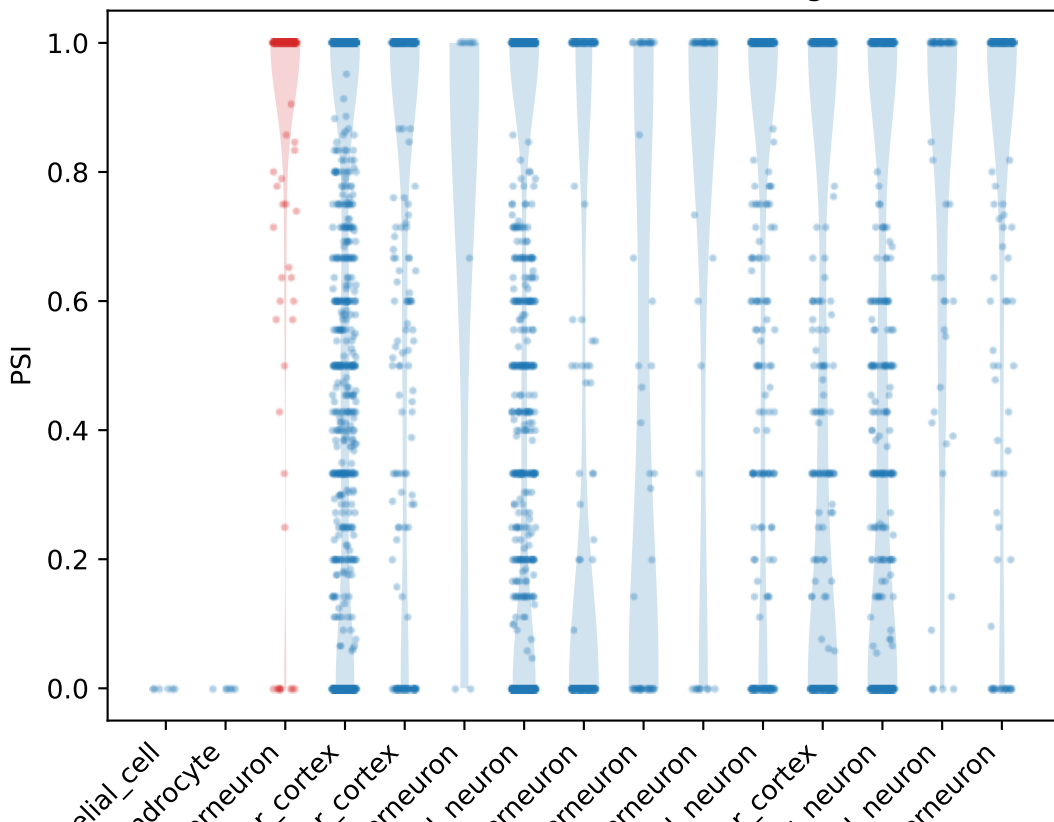
PSI distribution for Mff ProteinCoding7 exon
