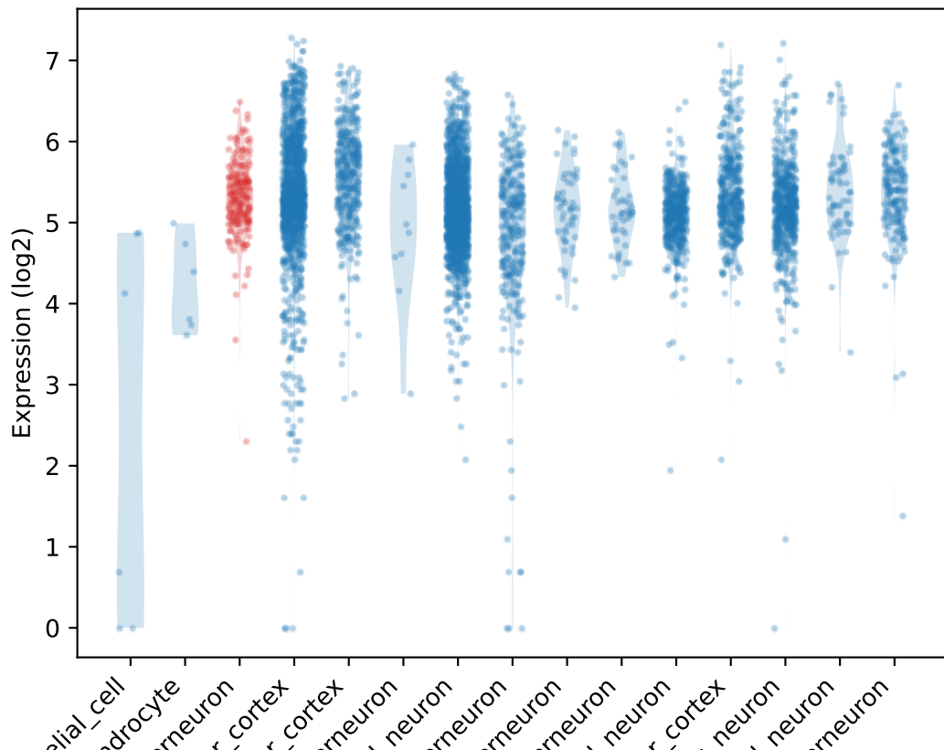
Count distribution for Mff
