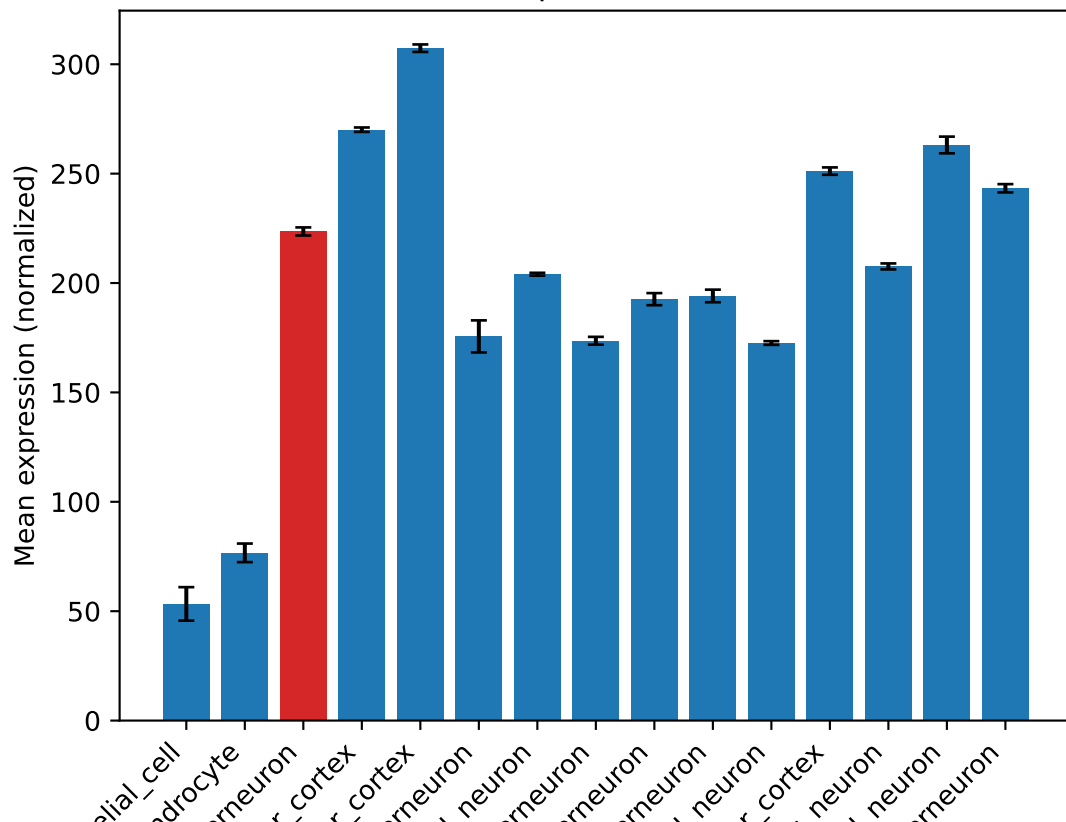
Gene expression for Mff
