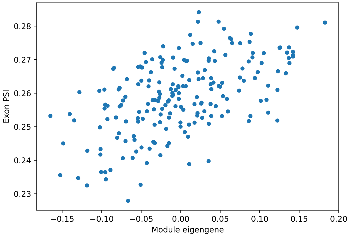
pvalb_GABAergic_cortical_interneuron ME vs. PSI for Mff other1 exon Corr: 0.55
