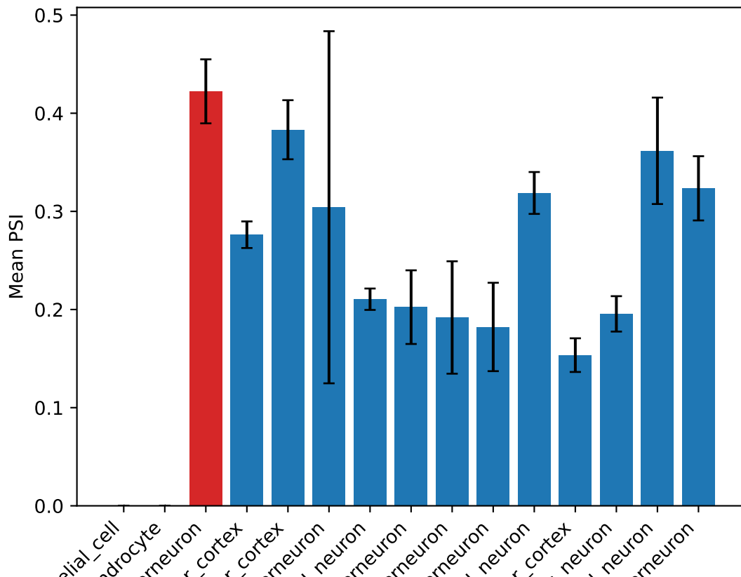
PSI for Mff other1 exon
