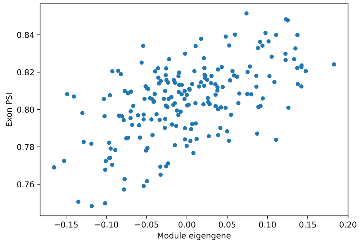
pvalb_GABAergic_cortical_interneuron ME vs. PSI for Rragb ProteinCoding1 c Corr: 0.57
