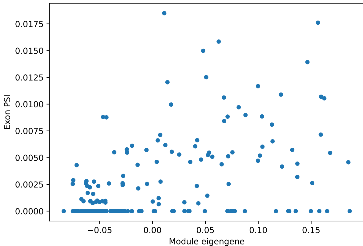
sncg_GABAergic_cortical_interneuron ME vs. PSI for Erc1 ProteinCoding3 Corr: 0.49
