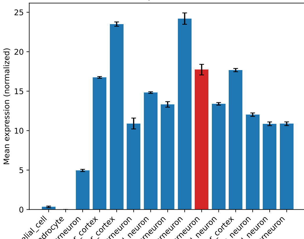
Gene expression for Erc1
