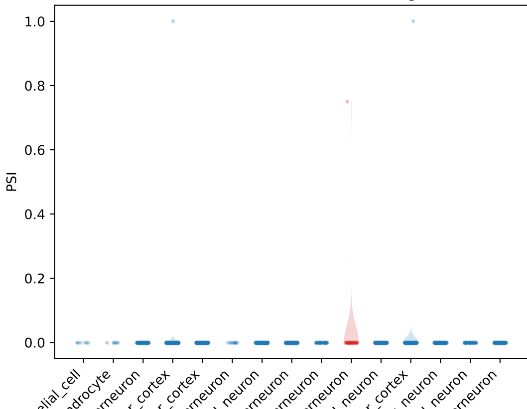
PSI distribution for Erc1 ProteinCoding3 exon
