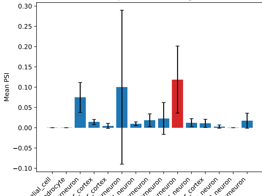
PSI for Impdh1 ProteinCoding1 exon
