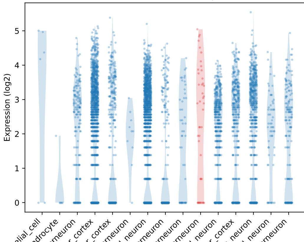
Count distribution for Impdh1
