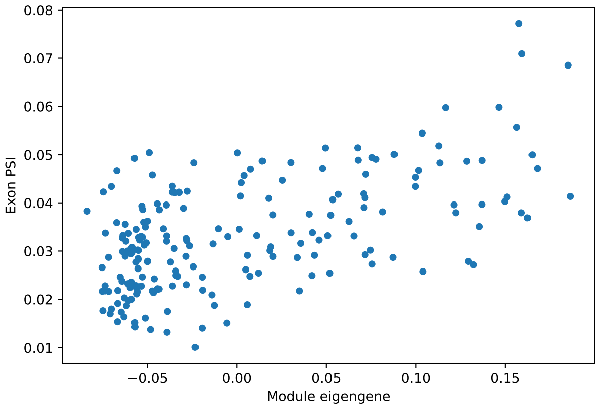
sncg_GABAergic_cortical_interneuron ME vs. PSI for Impdh1 ProteinCoding1 Corr: 0.58
