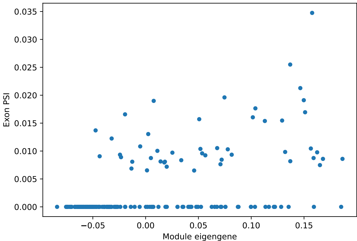
sncg_GABAergic_cortical_interneuron ME vs. PSI for Map2 ProteinCoding5 Corr: 0.52
