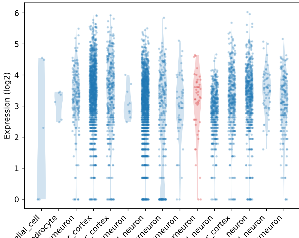
Count distribution for Spag9
