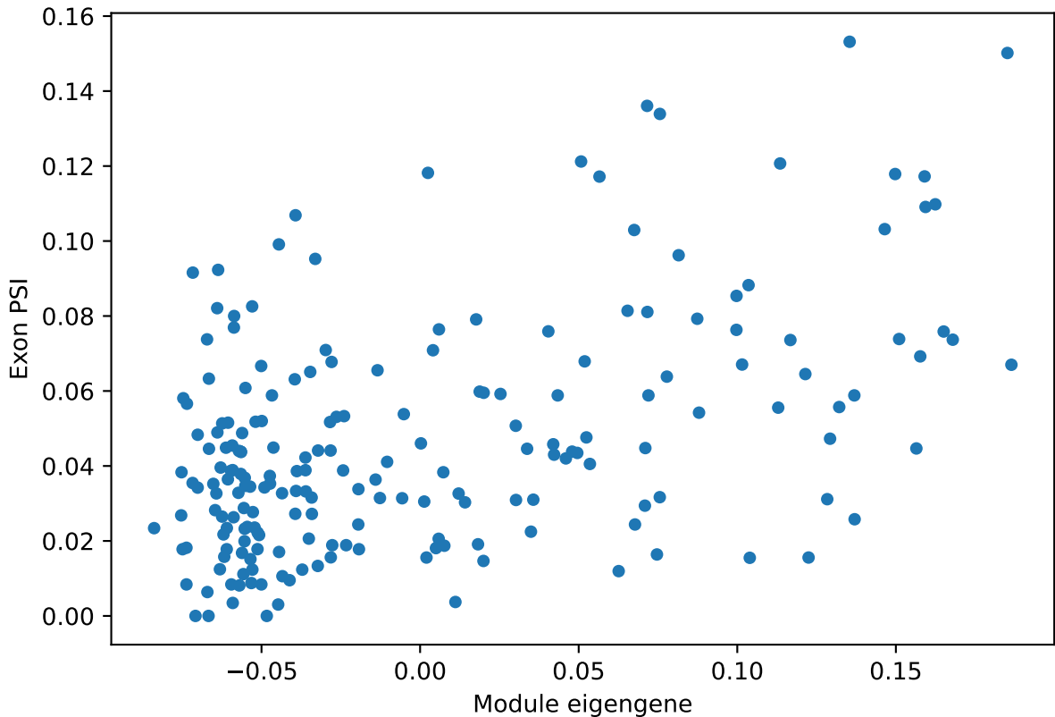
sncg_GABAergic_cortical_interneuron ME vs. PSI for Spag9 ProteinCoding5 Corr: 0.49
