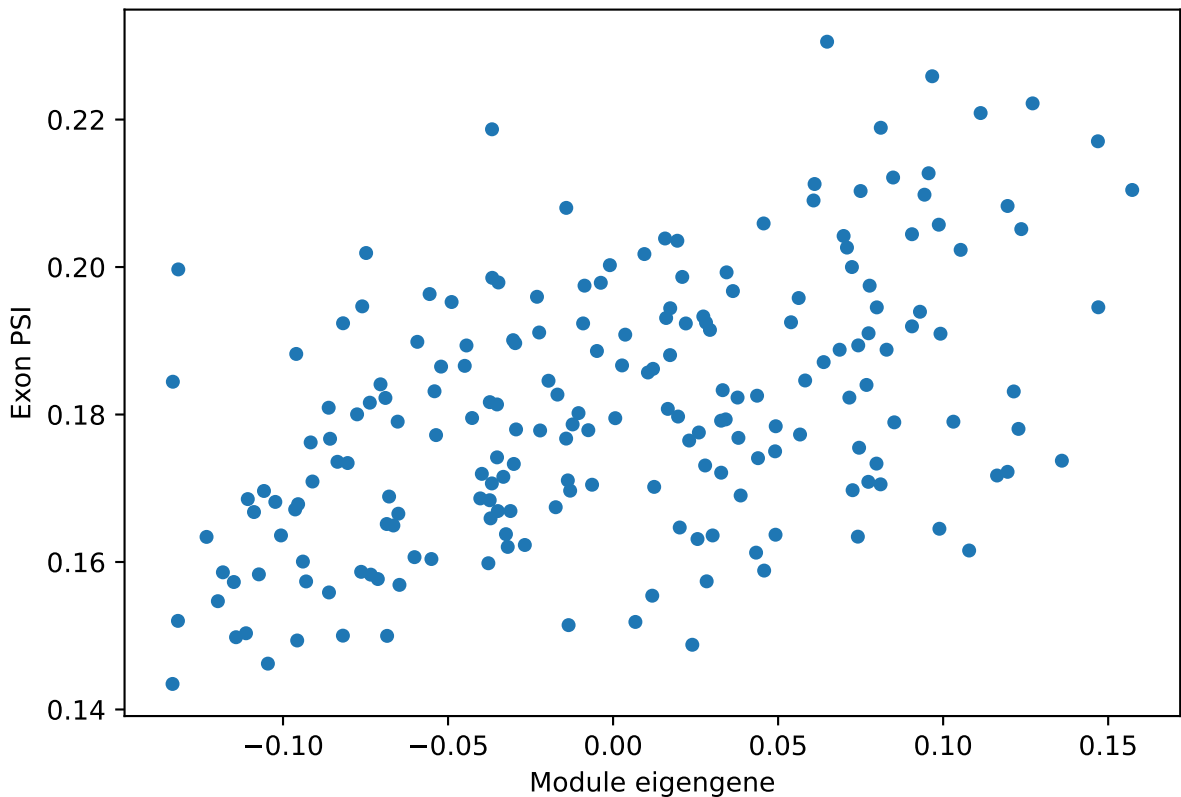
sst_GABAergic_cortical_interneuron ME vs. PSI for Ncam1 ProteinCoding1 (Corr: 0.5)
