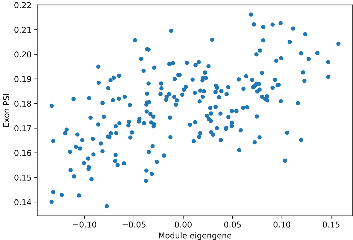
sst_GABAergic_cortical_interneuron ME vs. PSI for Sars1 ProteinCoding1 e Corr: 0.54
