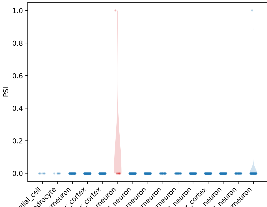
PSI distribution for Glis1 other1 exon
