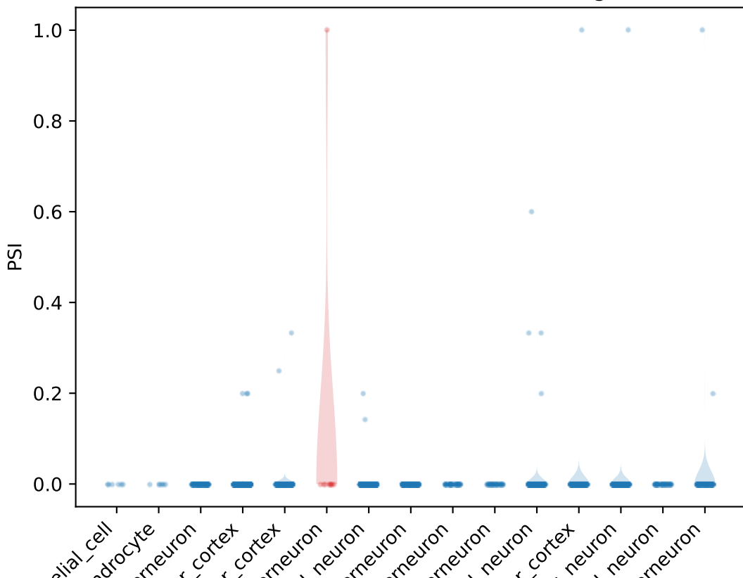
PSI distribution for Zswim1 ProteinCoding1 exon
