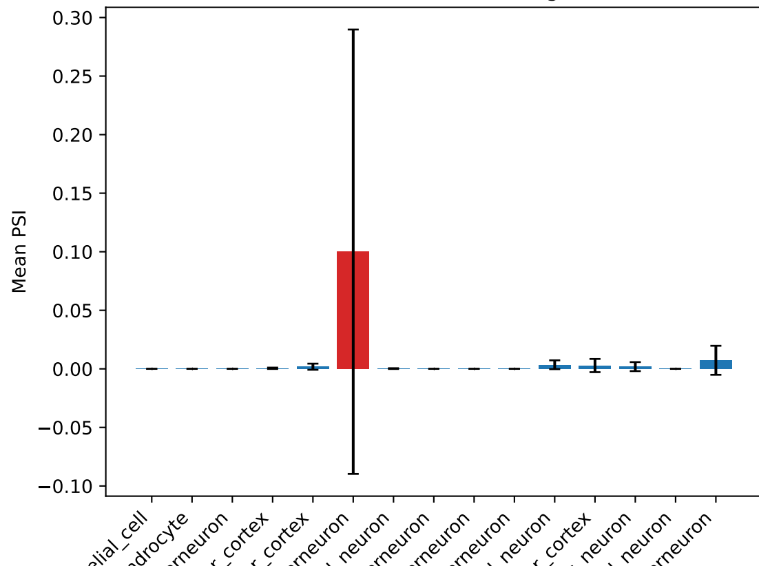
PSI for Zswim1 ProteinCoding1 exon
