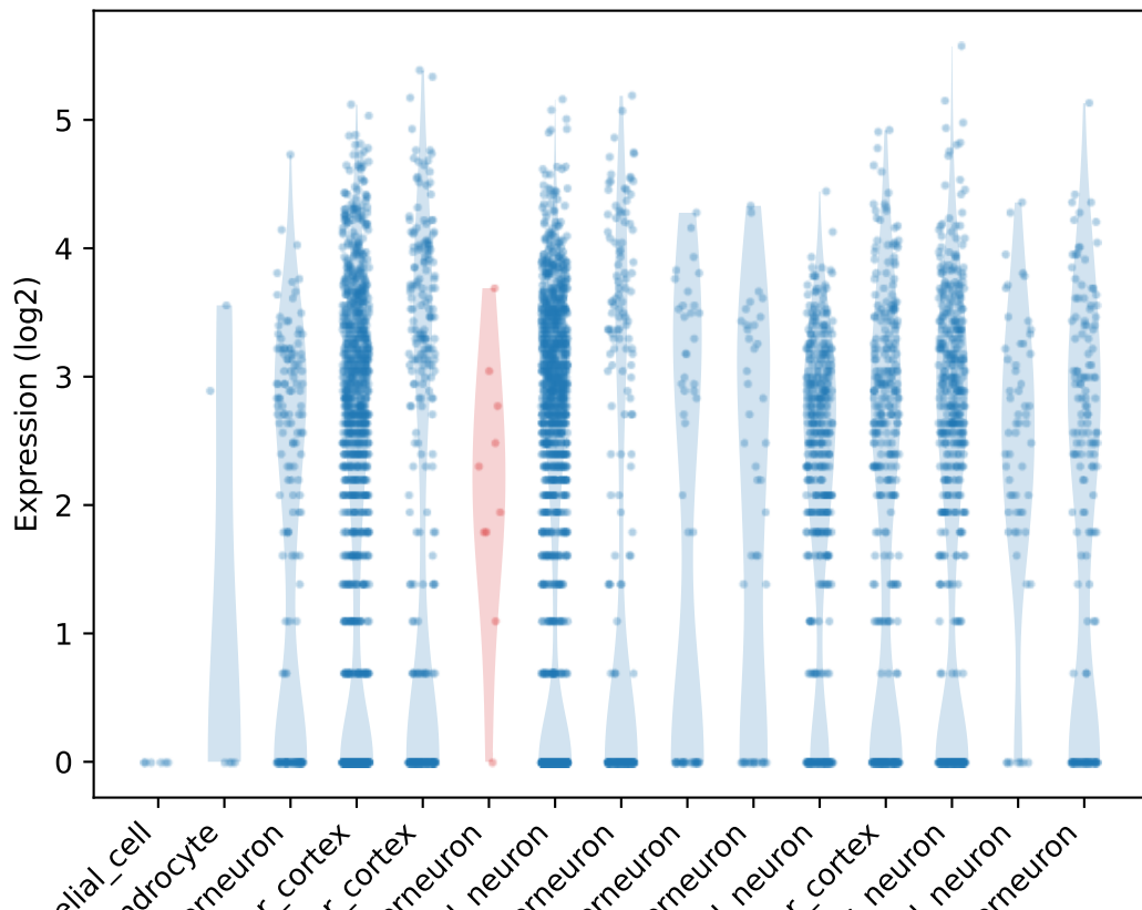
Count distribution for Zswim1
