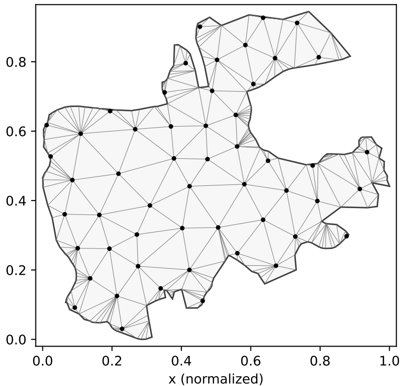
(b) Initial CDT: 276 vertices, 326 triangles
