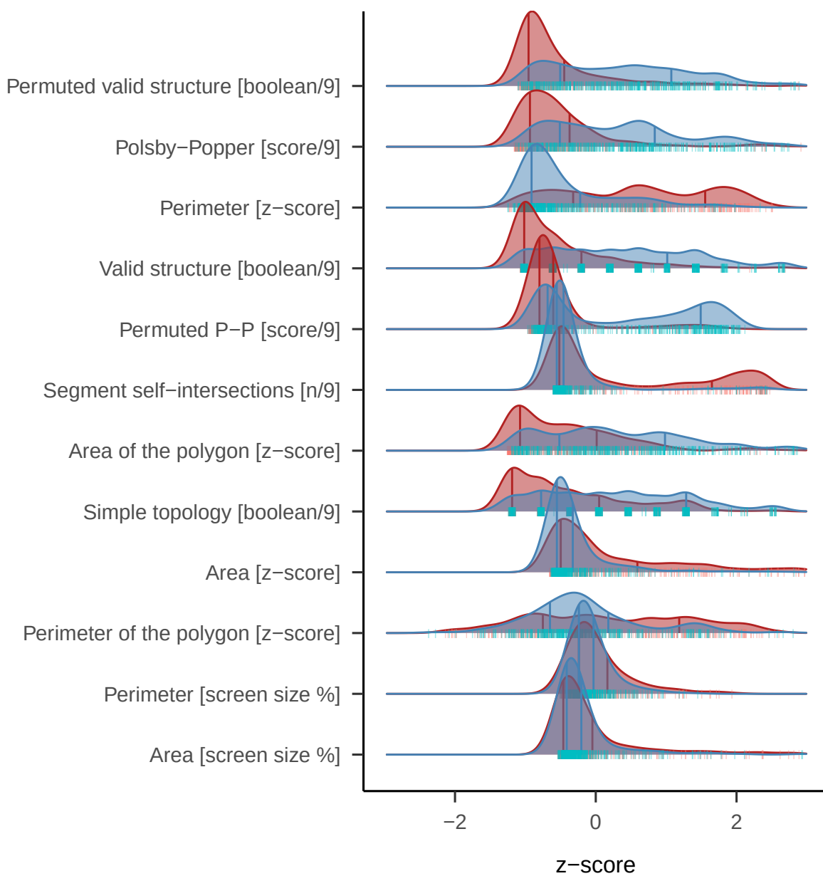
Method
