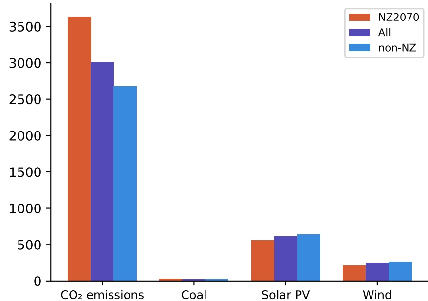
RMSE
