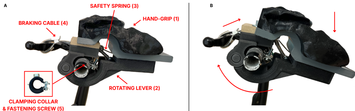
Figure 1: VeloBrake Assist. A. Components B. Activation movement
