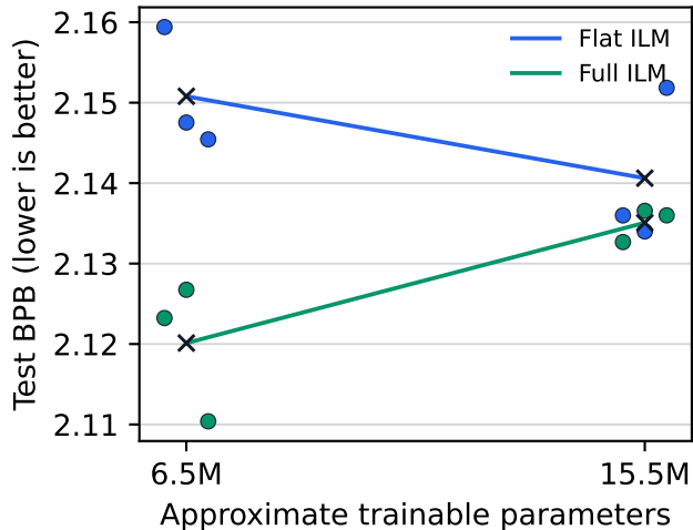
Tiny Shakespeare
