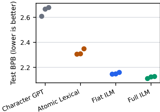
Tiny Shakespeare
