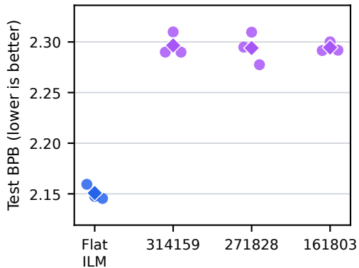
Tiny Shakespeare
