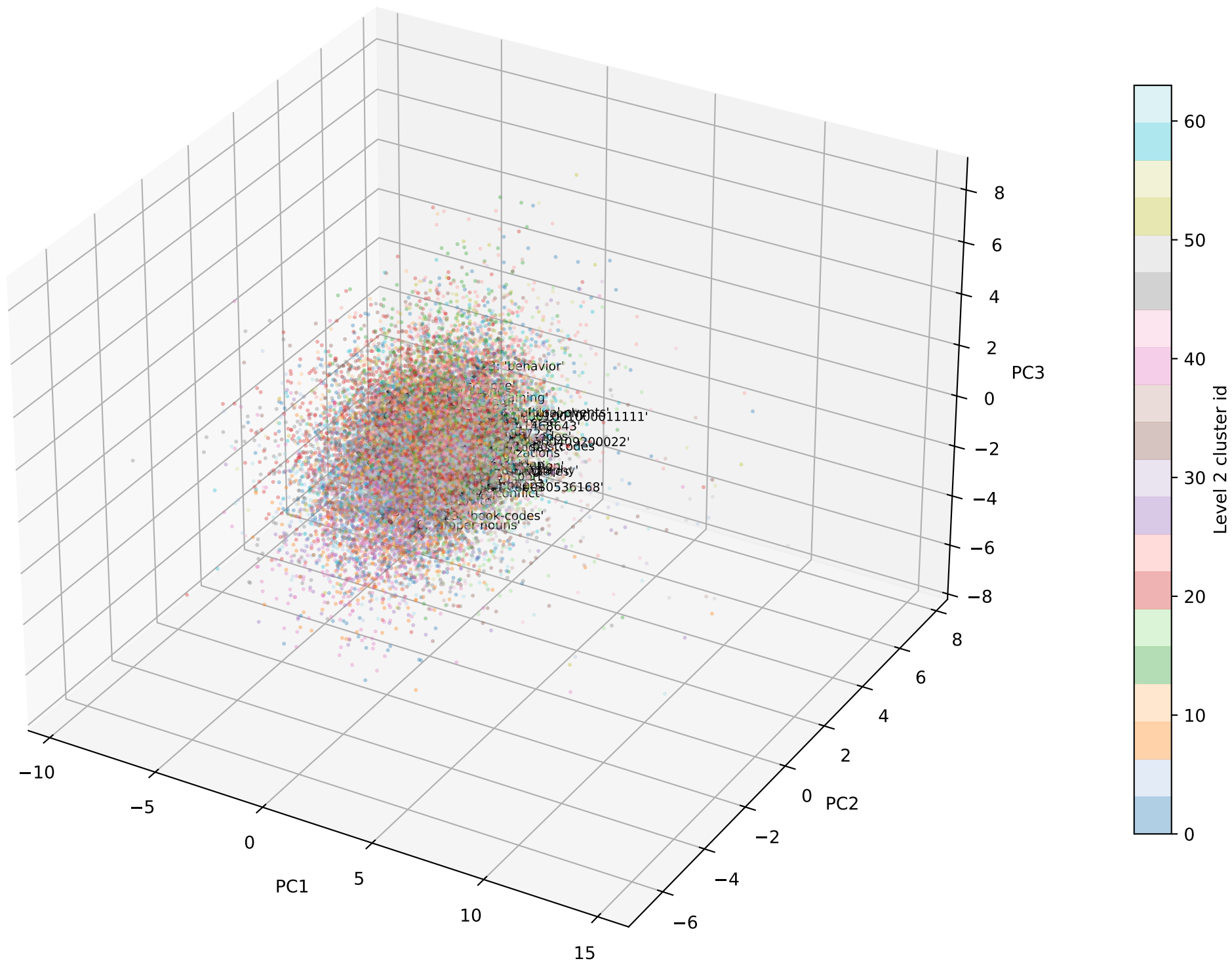
✗ Level 2 centroids
